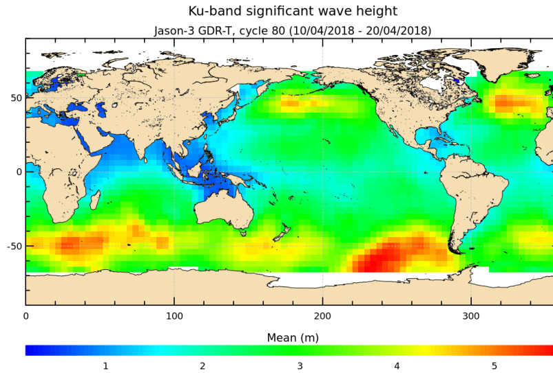
FIGURE 5 – Significant wave height for cycle 080.
