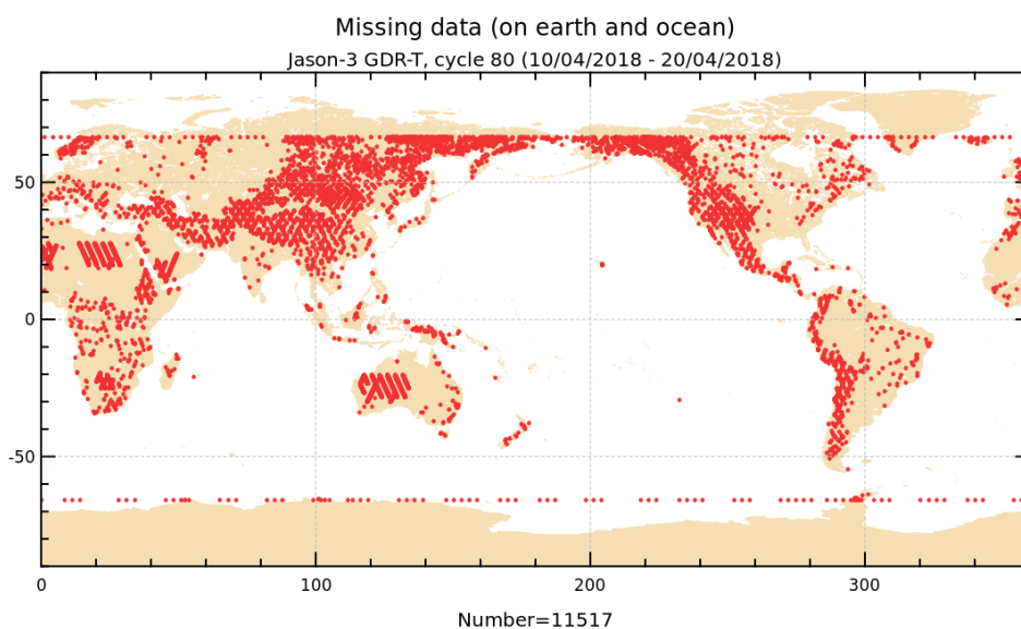
FIGURE 1 – Missing measurements for cycle 080.
