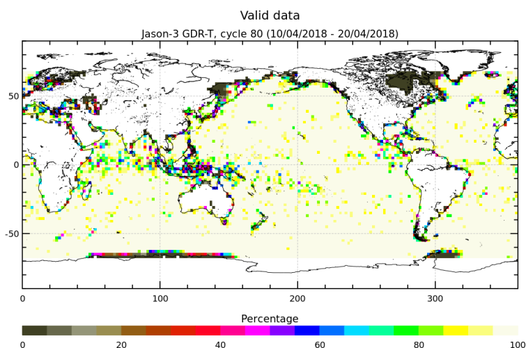
FIGURE 3 – Percentage of valid measurements for cycle 080.
