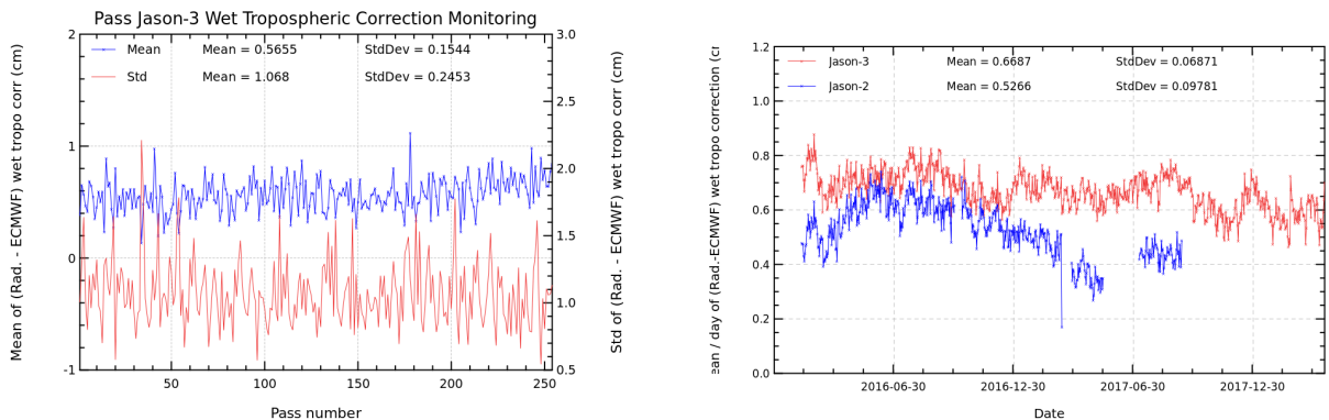
FIGURE 11 – Pass monitoring of wet troposphere differences between radiometer and ECMWF model for Jason-3 cycle 080 (left) and Jason-3 versus Jason-2 daily monitoring of wet troposphere differences between radiometer and ECMWF model (right).
