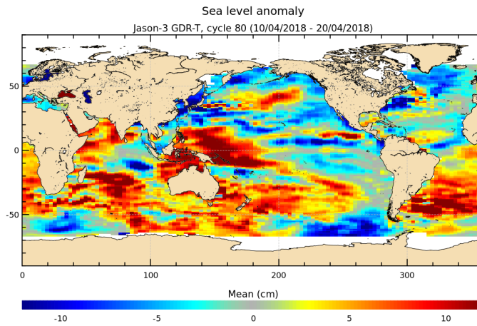
FIGURE 17 – Sea level anomaly relative to MSS for cycle 080.
