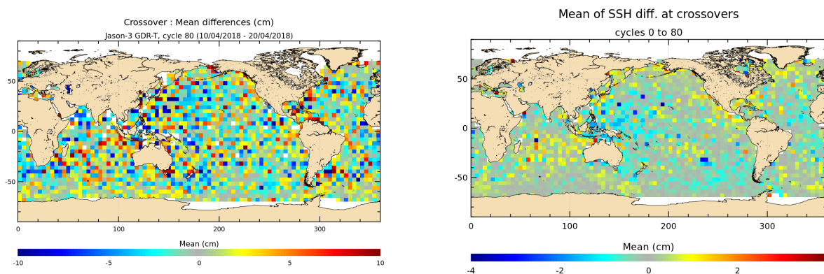
FIGURE 12 – Mean SSH at crossovers for cycle 080 (left) and over the whole Jason-3 period (right).
