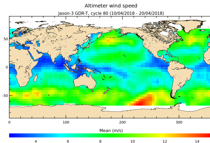
FIGURE 9 – Altimeter wind speed for cycle 080.
