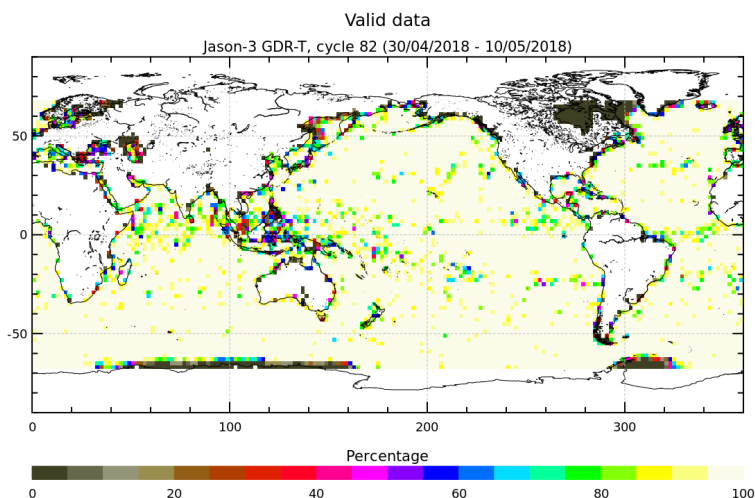
FIGURE 3 – Percentage of valid measurements for cycle 082.
