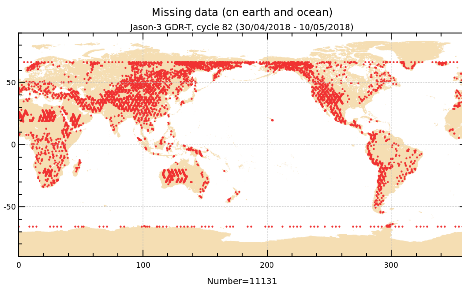
FIGURE 1 – Missing measurements for cycle 082.
