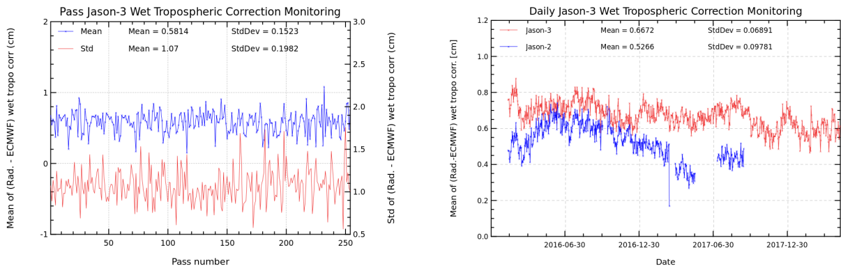
FIGURE 11 – Pass monitoring of wet troposphere differences between radiometer and ECMWF model for Jason-3 cycle 082 (left) and Jason-3 versus Jason-2 daily monitoring of wet troposphere differences between radiometer and ECMWF model (right).
