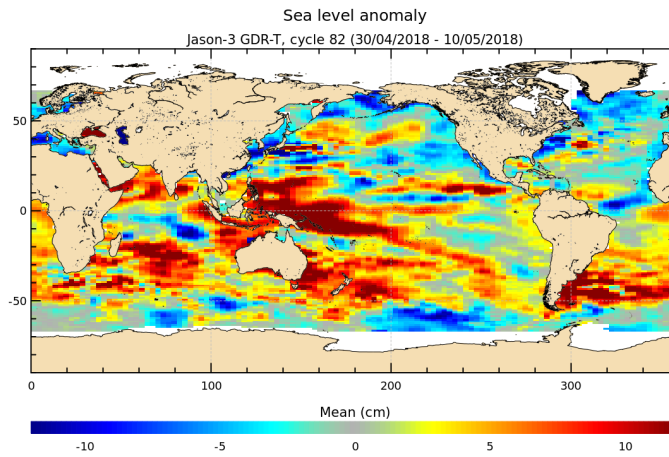
FIGURE 17 – Sea level anomaly relative to MSS for cycle 082.
