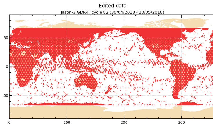
FIGURE 2 – Edited measurements for cycle 082.
