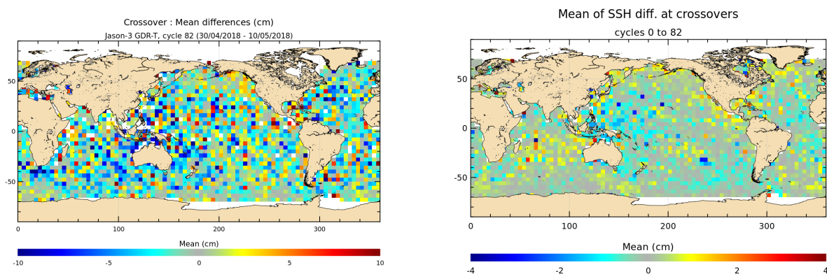
FIGURE 12 – Mean SSH at crossovers for cycle 082 (left) and over the whole Jason-3 period (right).
