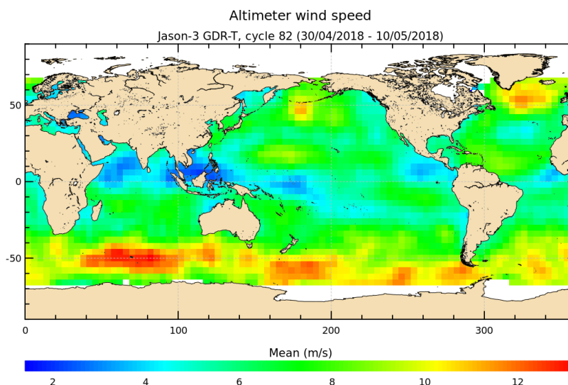
FIGURE 9 – Altimeter wind speed for cycle 082.
