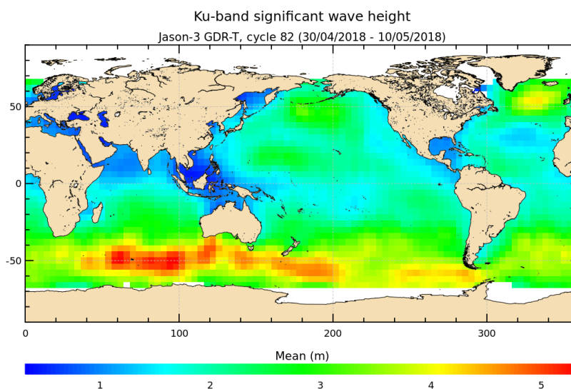
FIGURE 5 – Significant wave height for cycle 082.
