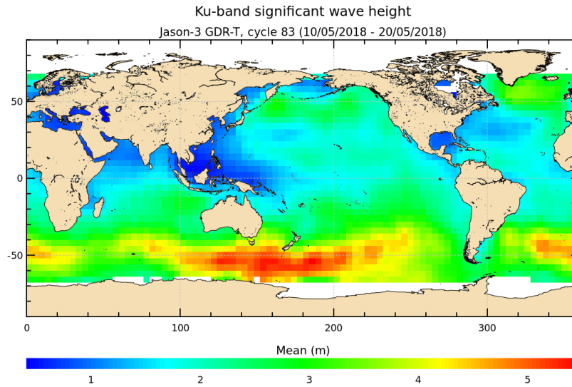
FIGURE 5 – Significant wave height for cycle 083.
