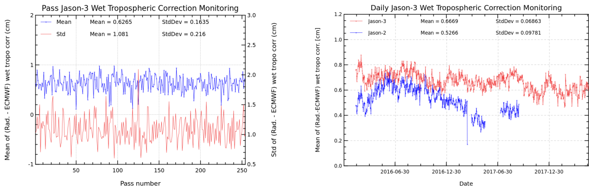
FIGURE 11 – Pass monitoring of wet troposphere differences between radiometer and ECMWF model for Jason-3 cycle 083 (left) and Jason-3 versus Jason-2 daily monitoring of wet troposphere differences between radiometer and ECMWF model (right).
