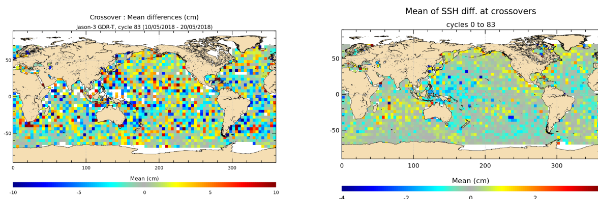
FIGURE 12 – Mean SSH at crossovers for cycle 083 (left) and over the whole Jason-3 period (right).
