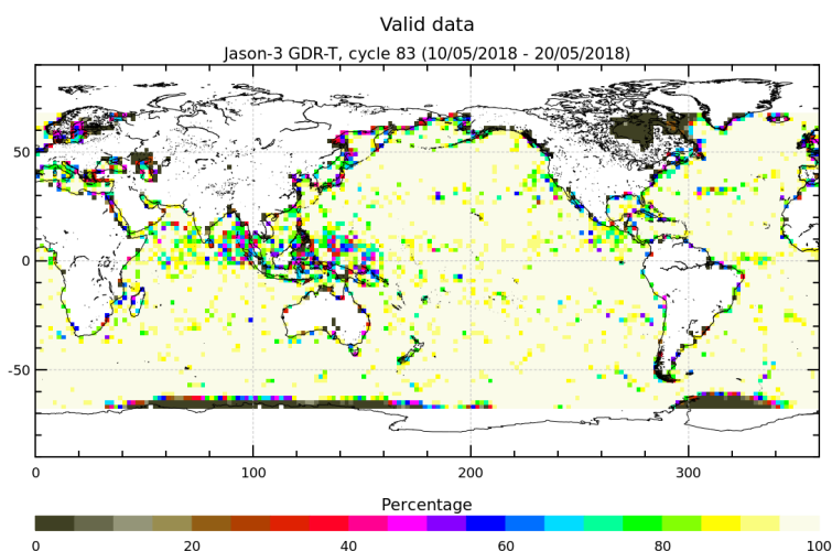
FIGURE 3 – Percentage of valid measurements for cycle 083.
