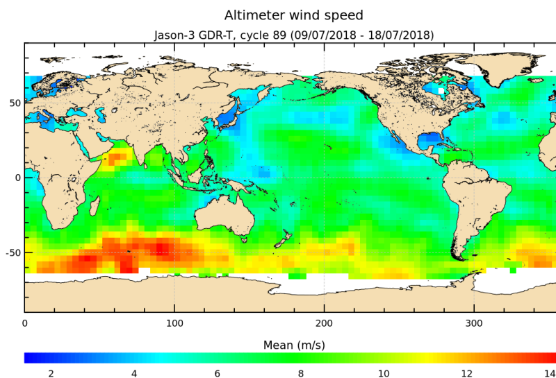
FIGURE 9 – Altimeter wind speed for cycle 089.
