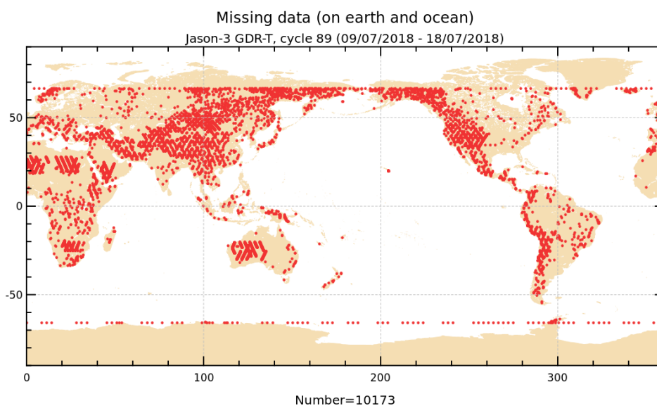
FIGURE 1 – Missing measurements for cycle 089.
