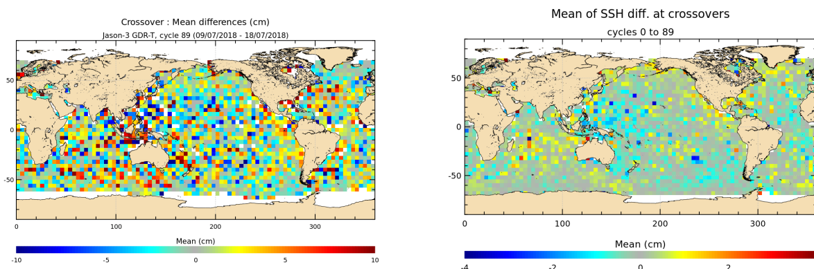
FIGURE 12 – Mean SSH at crossovers for cycle 089 (left) and over the whole Jason-3 period (right).
