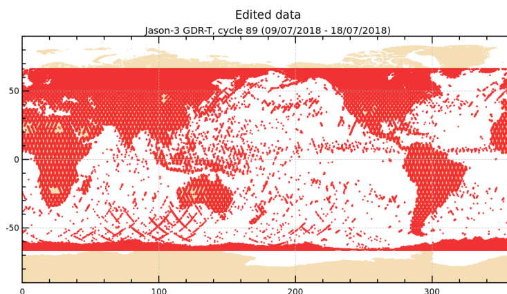
FIGURE 2 – Edited measurements for cycle 089.
