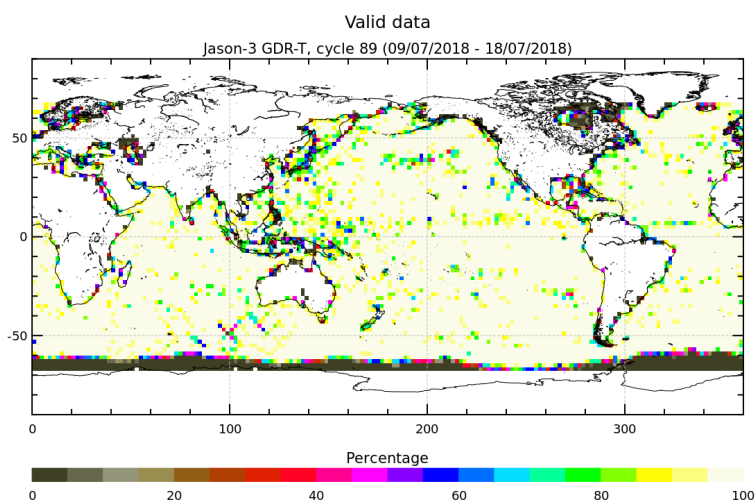
FIGURE 3 – Percentage of valid measurements for cycle 089.
