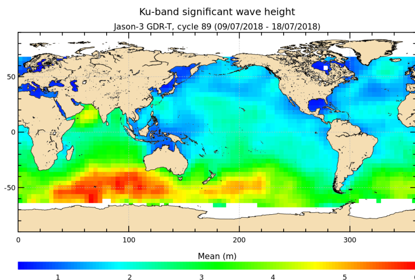
FIGURE 5 – Significant wave height for cycle 089.
