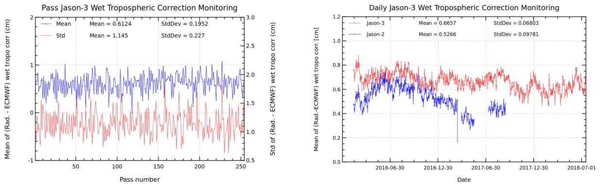
FIGURE 11 – Pass monitoring of wet troposphere differences between radiometer and ECMWF model for Jason-3 cycle 089 (left) and Jason-3 versus Jason-2 daily monitoring of wet troposphere differences between radiometer and ECMWF model (right).
