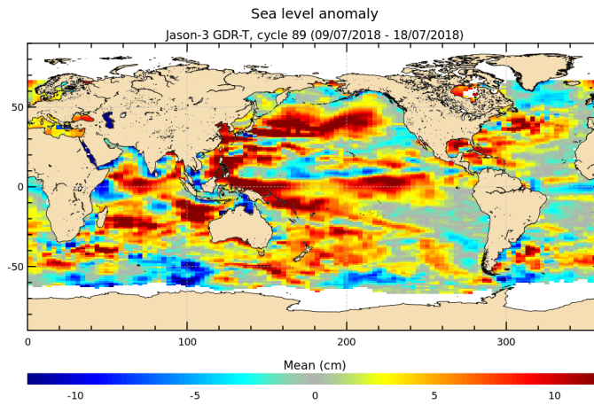
FIGURE 17 – Sea level anomaly relative to MSS for cycle 089.
