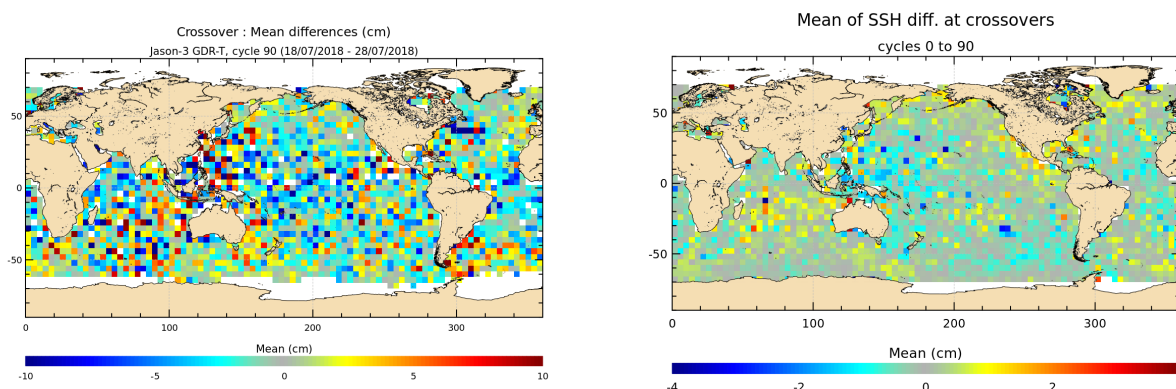
FIGURE 12 – Mean SSH at crossovers for cycle 090 (left) and over the whole Jason-3 period (right).
