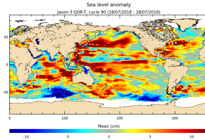
FIGURE 17 – Sea level anomaly relative to MSS for cycle 090.
