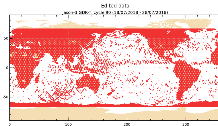
FIGURE 2 – Edited measurements for cycle 090.
