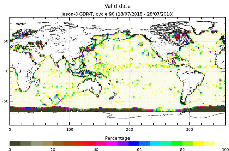
FIGURE 3 – Percentage of valid measurements for cycle 090.
