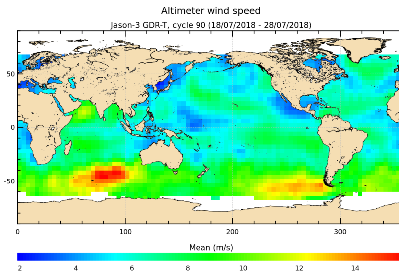
FIGURE 9 – Altimeter wind speed for cycle 090.
