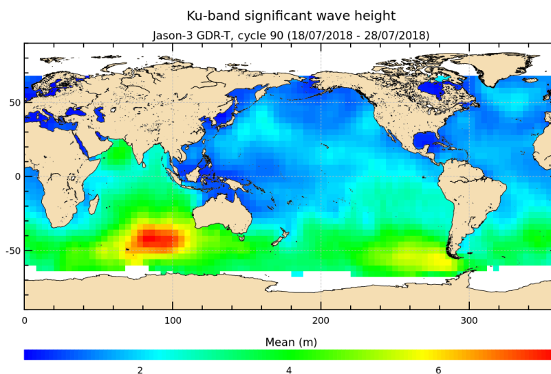
FIGURE 5 – Significant wave height for cycle 090.
