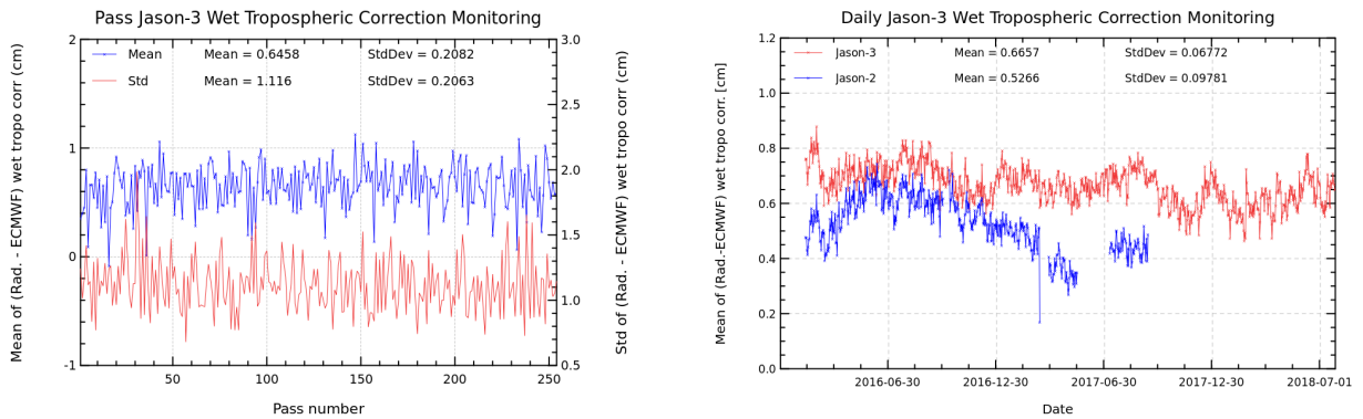
FIGURE 11 – Pass monitoring of wet troposphere differences between radiometer and ECMWF model for Jason-3 cycle 090 (left) and Jason-3 versus Jason-2 daily monitoring of wet troposphere differences between radiometer and ECMWF model (right).
