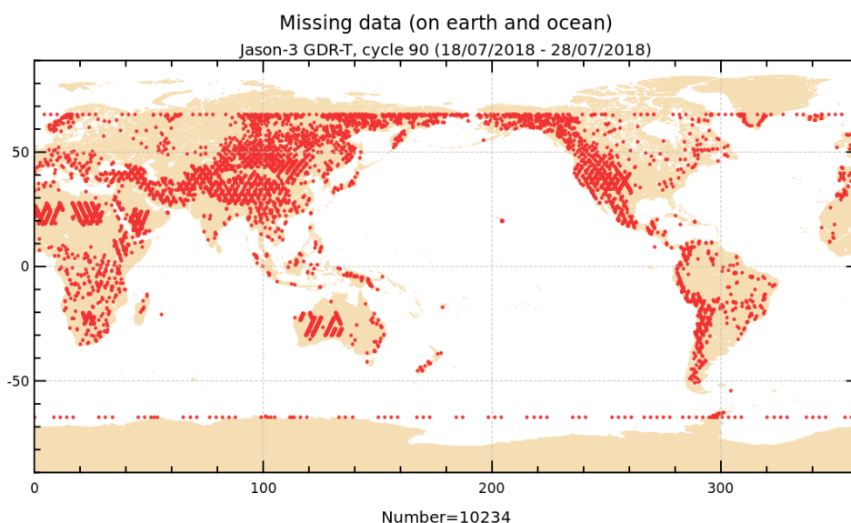
FIGURE 1 – Missing measurements for cycle 090.
