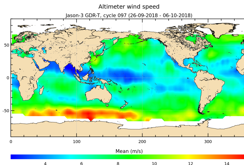
FIGURE 9 – Altimeter wind speed for cycle 097.
