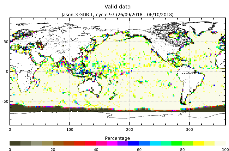
FIGURE 3 – Percentage of valid measurements for cycle 097.
