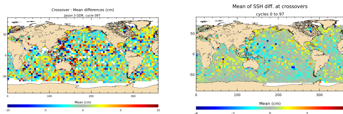
FIGURE 12 – Mean SSH at crossovers for cycle 097 (left) and over the whole Jason-3 period (right).
