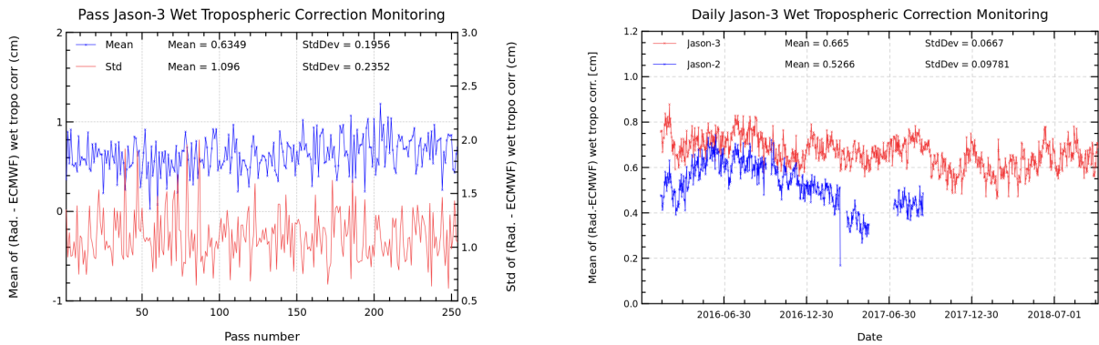
FIGURE 11 – Pass monitoring of wet troposphere differences between radiometer and ECMWF model for Jason-3 cycle 097 (left) and Jason-3 versus Jason-2 daily monitoring of wet troposphere differences between radiometer and ECMWF model (right).
