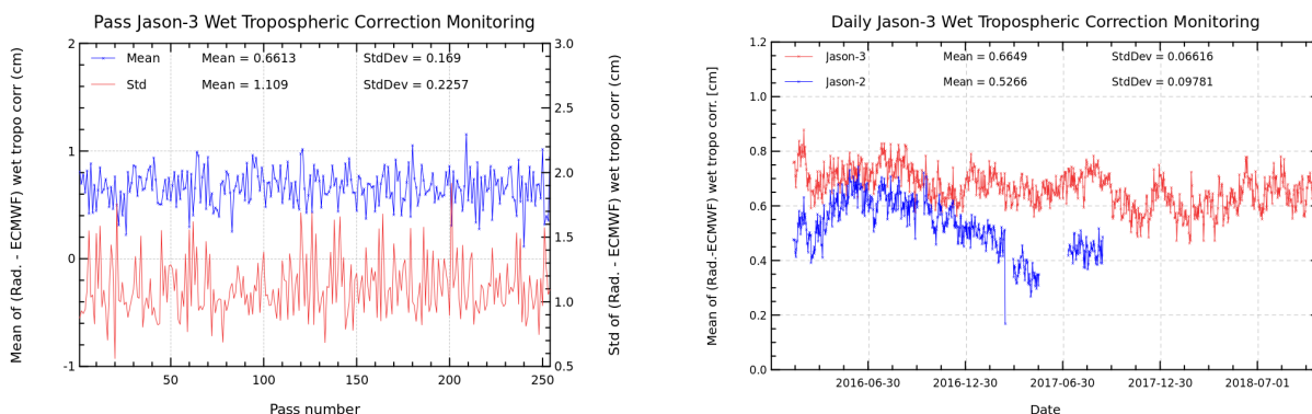
FIGURE 11 – Pass monitoring of wet troposphere differences between radiometer and ECMWF model for Jason-3 cycle 099 (left) and Jason-3 versus Jason-2 daily monitoring of wet troposphere differences between radiometer and ECMWF model (right).
