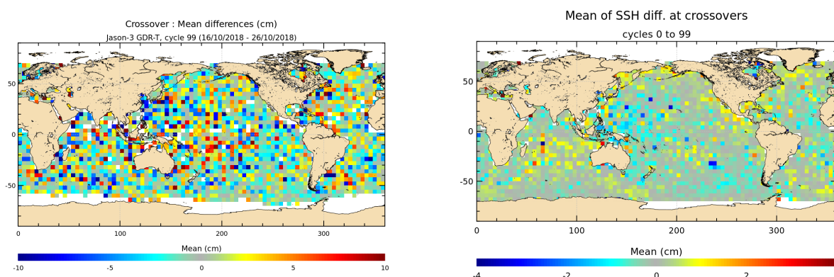
FIGURE 12 – Mean SSH at crossovers for cycle 099 (left) and over the whole Jason-3 period (right).
