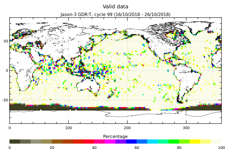
FIGURE 3 – Percentage of valid measurements for cycle 099.
