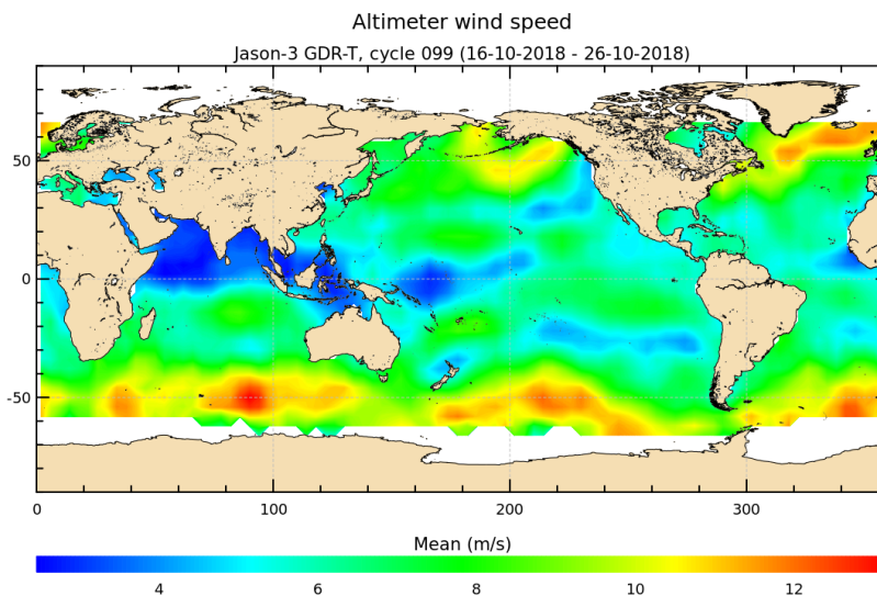
FIGURE 9 – Altimeter wind speed for cycle 099.
