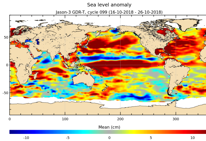
FIGURE 17 – Sea level anomaly relative to MSS for cycle 099.
