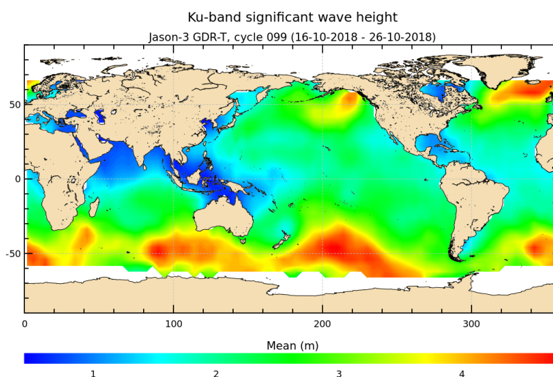
FIGURE 5 – Significant wave height for cycle 099.
