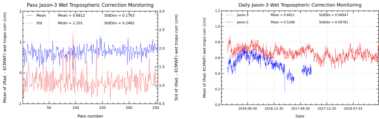
FIGURE 11 – Pass monitoring of wet troposphere differences between radiometer and ECMWF model for Jason-3 cycle 105 (left) and Jason-3 versus Jason-2 daily monitoring of wet troposphere differences between radiometer and ECMWF model (right).
