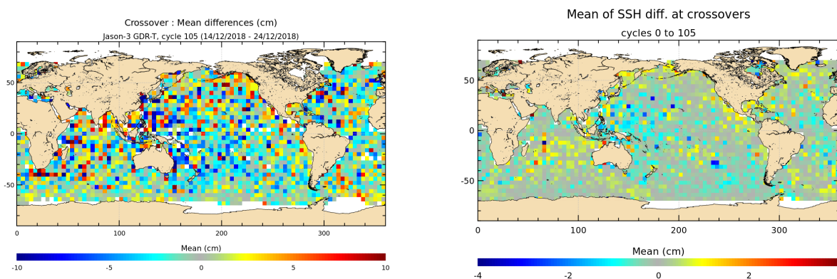
FIGURE 12 – Mean SSH at crossovers for cycle 105 (left) and over the whole Jason-3 period (right).
