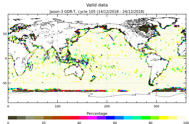
FIGURE 3 – Percentage of valid measurements for cycle 105.
