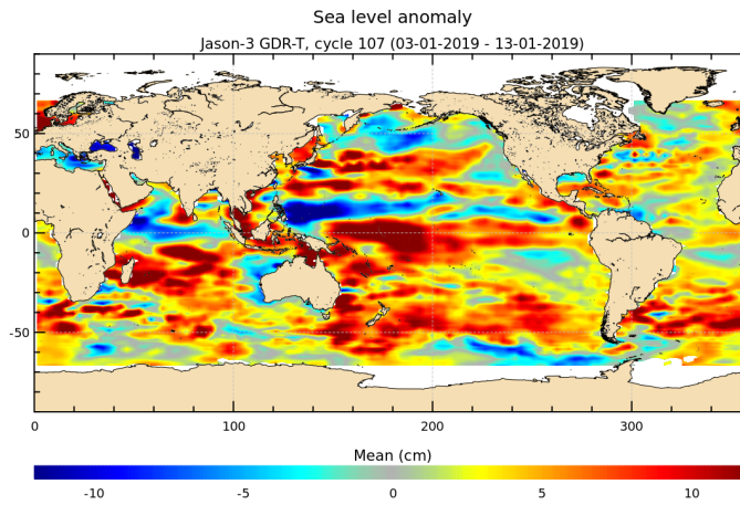
FIGURE 17 – Sea level anomaly relative to MSS for cycle 107.
