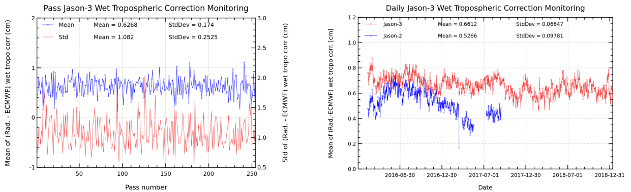
FIGURE 11 – Pass monitoring of wet troposphere differences between radiometer and ECMWF model for Jason-3 cycle 107 (left) and Jason-3 versus Jason-2 daily monitoring of wet troposphere differences between radiometer and ECMWF model (right).
