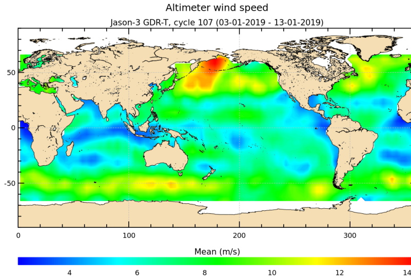
FIGURE 9 – Altimeter wind speed for cycle 107.
