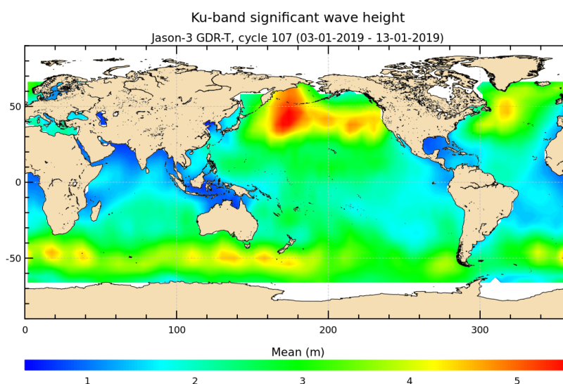
FIGURE 5 – Significant wave height for cycle 107.
