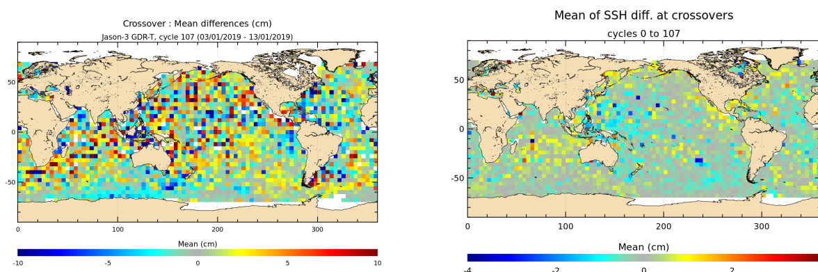
FIGURE 12 – Mean SSH at crossovers for cycle 107 (left) and over the whole Jason-3 period (right).
