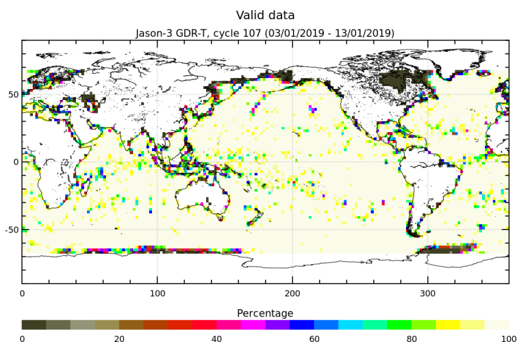
FIGURE 3 – Percentage of valid measurements for cycle 107.
