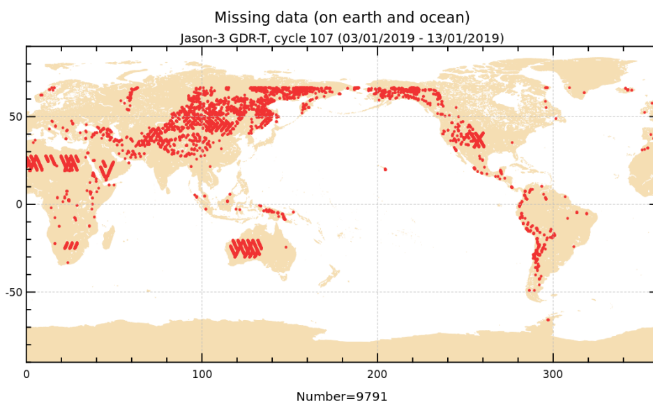
FIGURE 1 – Missing measurements for cycle 107.
