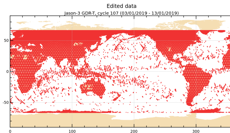
FIGURE 2 – Edited measurements for cycle 107.
