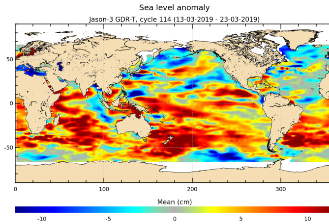
FIGURE 17 – Sea level anomaly relative to MSS for cycle 114.
