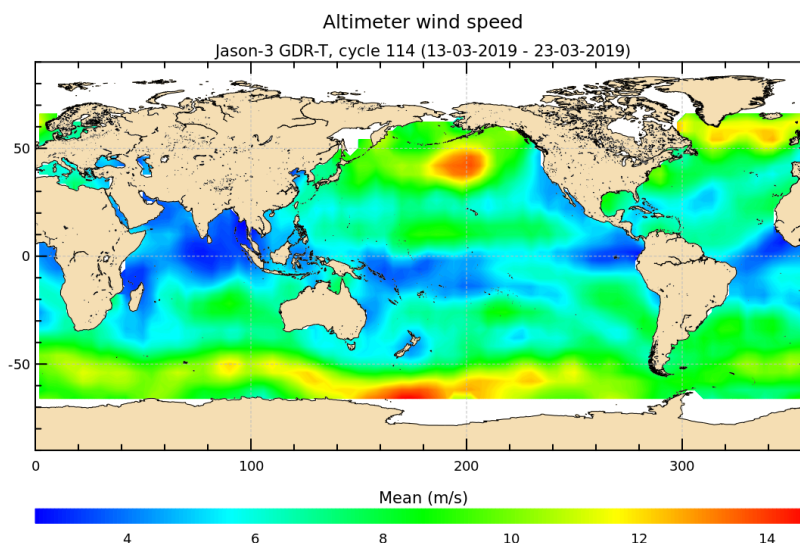
FIGURE 9 – Altimeter wind speed for cycle 114.
