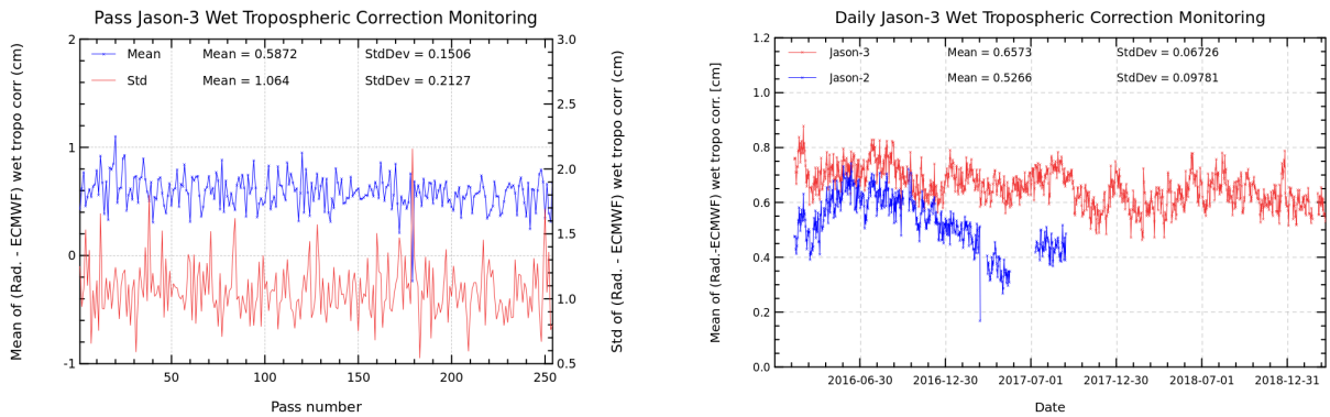
FIGURE 11 – Pass monitoring of wet troposphere differences between radiometer and ECMWF model for Jason-3 cycle 114 (left) and Jason-3 versus Jason-2 daily monitoring of wet troposphere differences between radiometer and ECMWF model (right).
