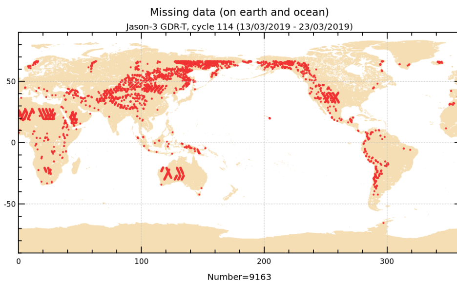
FIGURE 1 – Missing measurements for cycle 114.
