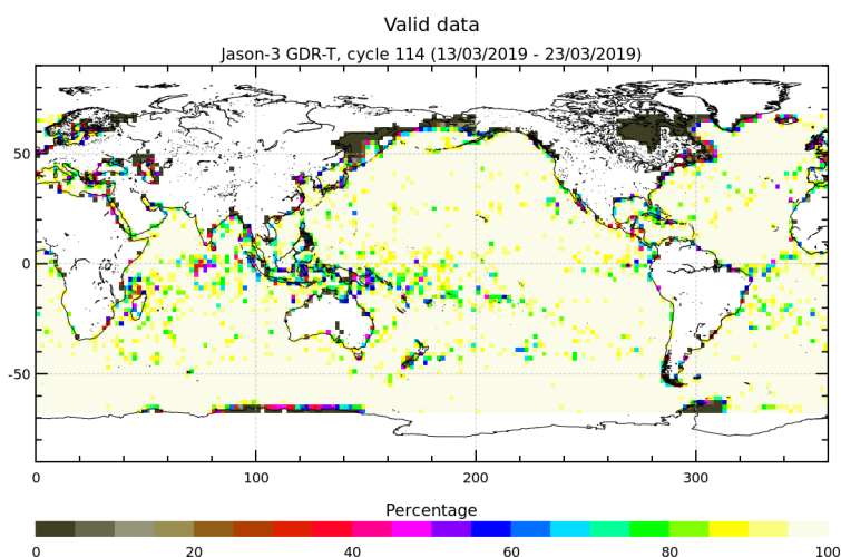
FIGURE 3 – Percentage of valid measurements for cycle 114.
