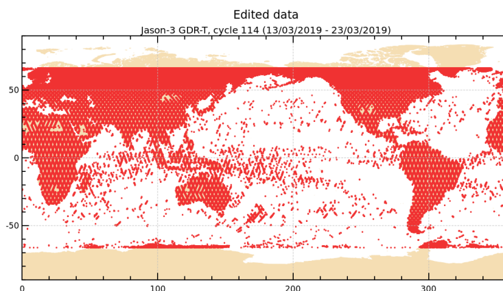
FIGURE 2 – Edited measurements for cycle 114.
