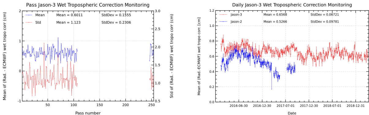
FIGURE 11 – Pass monitoring of wet troposphere differences between radiometer and ECMWF model for Jason-3 cycle 116 (left) and Jason-3 versus Jason-2 daily monitoring of wet troposphere differences between radiometer and ECMWF model (right).
