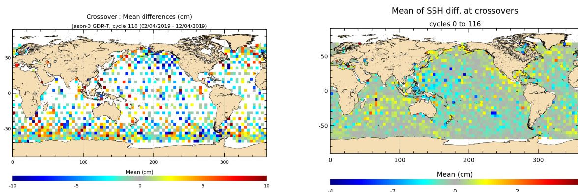
FIGURE 12 – Mean SSH at crossovers for cycle 116 (left) and over the whole Jason-3 period (right).
