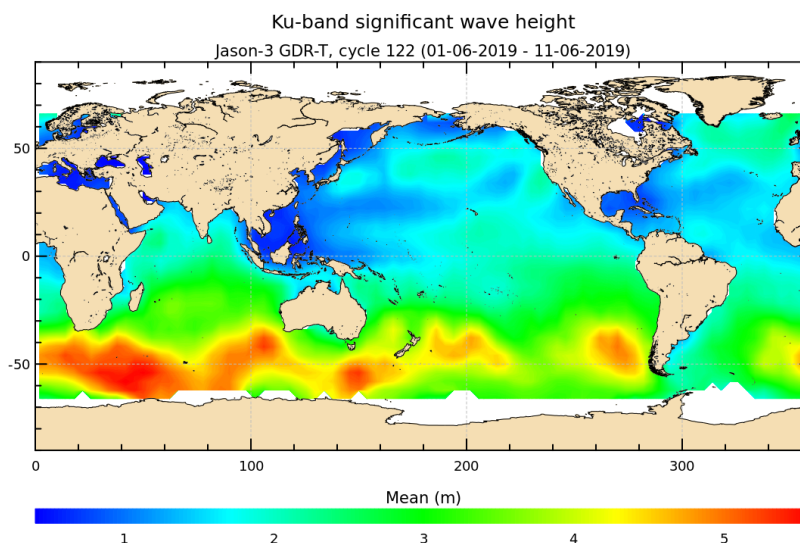
FIGURE 5 – Significant wave height for cycle 122.
