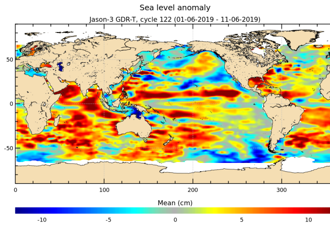
FIGURE 17 – Sea level anomaly relative to MSS for cycle 122.
