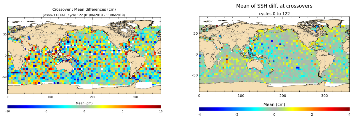
FIGURE 12 – Mean SSH at crossovers for cycle 122 (left) and over the whole Jason-3 period (right).
