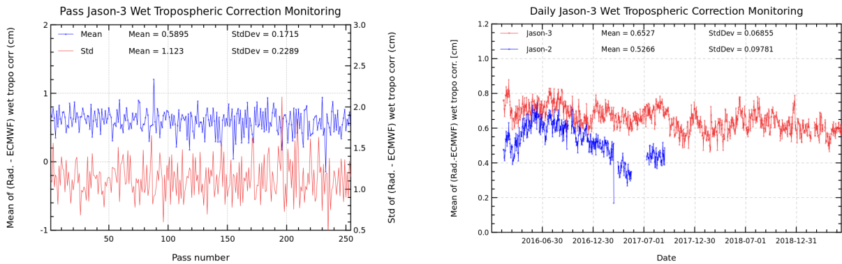
FIGURE 11 – Pass monitoring of wet troposphere differences between radiometer and ECMWF model for Jason-3 cycle 122 (left) and Jason-3 versus Jason-2 daily monitoring of wet troposphere differences between radiometer and ECMWF model (right).
