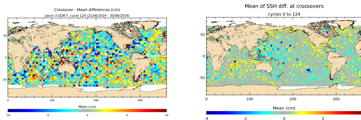
FIGURE 12 – Mean SSH at crossovers for cycle 124 (left) and over the whole Jason-3 period (right).
