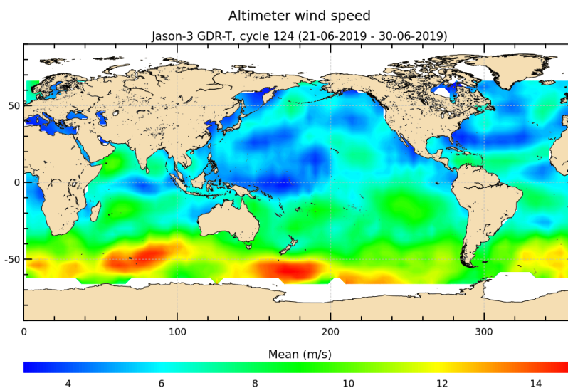
FIGURE 9 – Altimeter wind speed for cycle 124.
