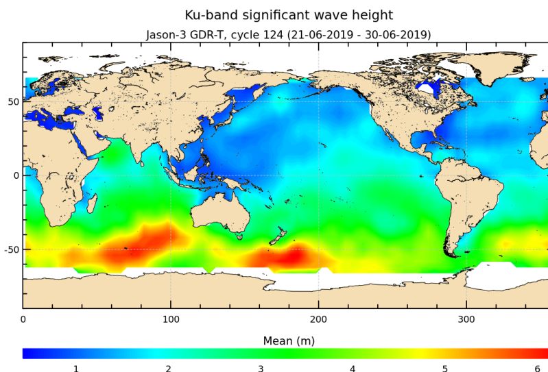
FIGURE 5 – Significant wave height for cycle 124.
