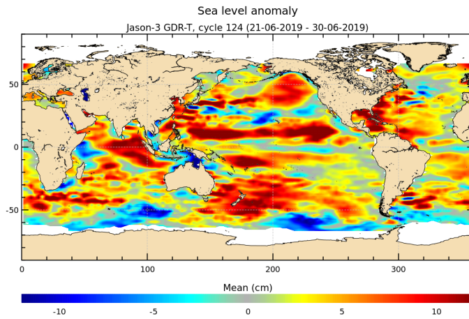
FIGURE 17 – Sea level anomaly relative to MSS for cycle 124.
