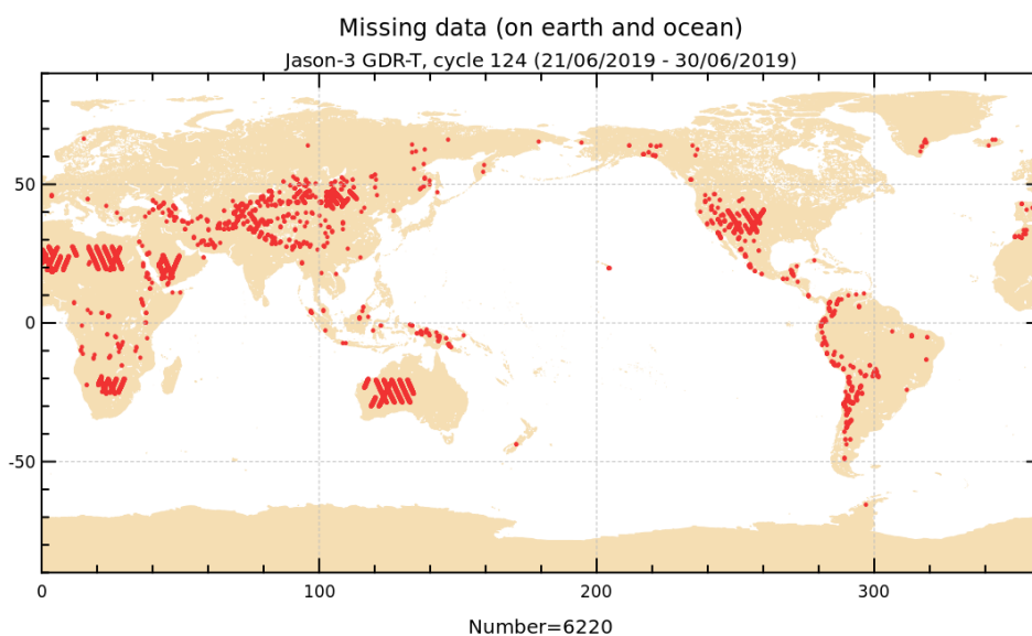
FIGURE 1 – Missing measurements for cycle 124.
