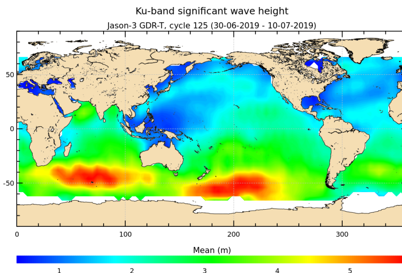
FIGURE 5 – Significant wave height for cycle 125.
