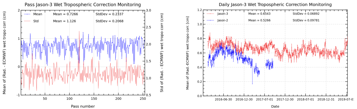
FIGURE 11 – Pass monitoring of wet troposphere differences between radiometer and ECMWF model for Jason-3 cycle 125 (left) and Jason-3 versus Jason-2 daily monitoring of wet troposphere differences between radiometer and ECMWF model (right).
