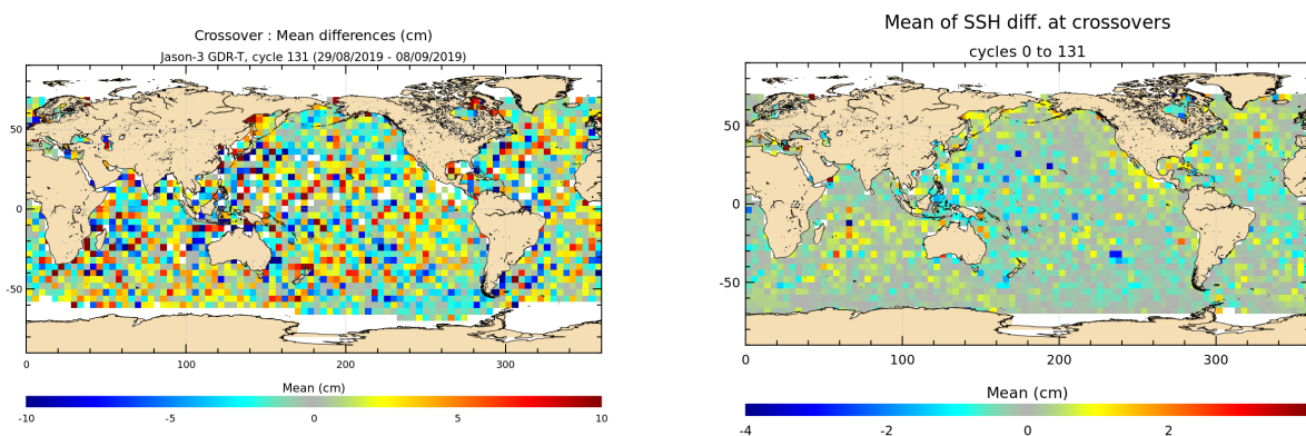
FIGURE 12 – Mean SSH at crossovers for cycle 131 (left) and over the whole Jason-3 period (right).
