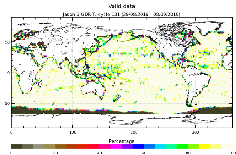
FIGURE 3 – Percentage of valid measurements for cycle 131.
