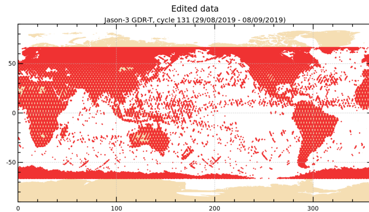
FIGURE 2 – Edited measurements for cycle 131.
