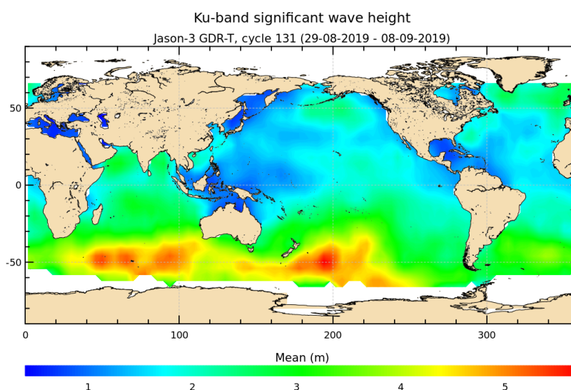
FIGURE 5 – Significant wave height for cycle 131.
