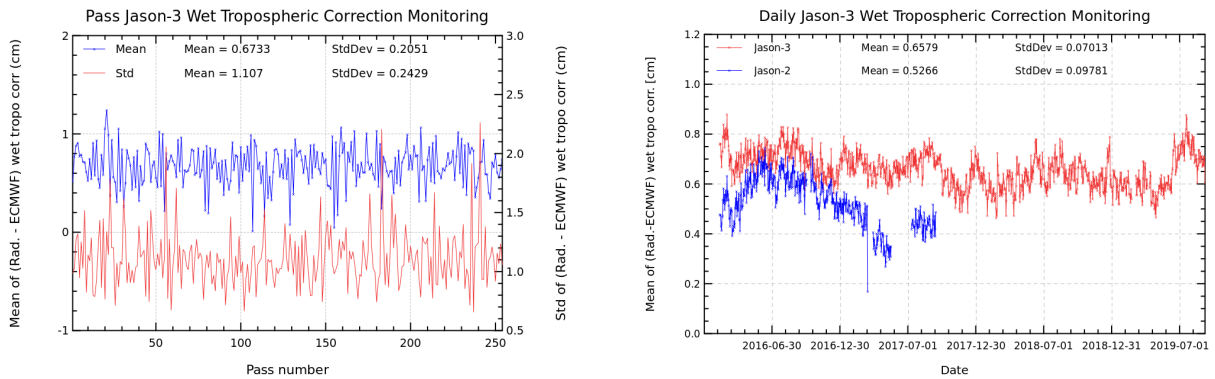
FIGURE 11 – Pass monitoring of wet troposphere differences between radiometer and ECMWF model for Jason-3 cycle 131 (left) and Jason-3 versus Jason-2 daily monitoring of wet troposphere differences between radiometer and ECMWF model (right).
