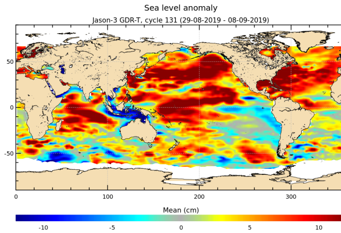
FIGURE 17 – Sea level anomaly relative to MSS for cycle 131.
