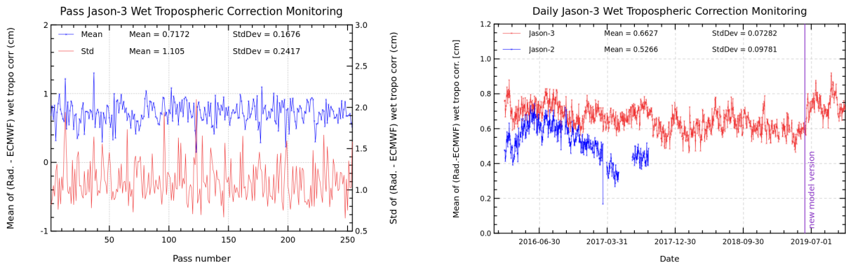
FIGURE 11 – Pass monitoring of wet troposphere differences between radiometer and ECMWF model for Jason-3 cycle 138 (left) and Jason-3 versus Jason-2 daily monitoring of wet troposphere differences between radiometer and ECMWF model (right).
