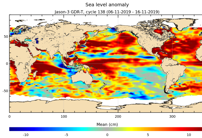
FIGURE 17 – Sea level anomaly relative to MSS for cycle 138.
