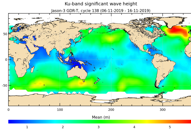
FIGURE 5 – Significant wave height for cycle 138.
