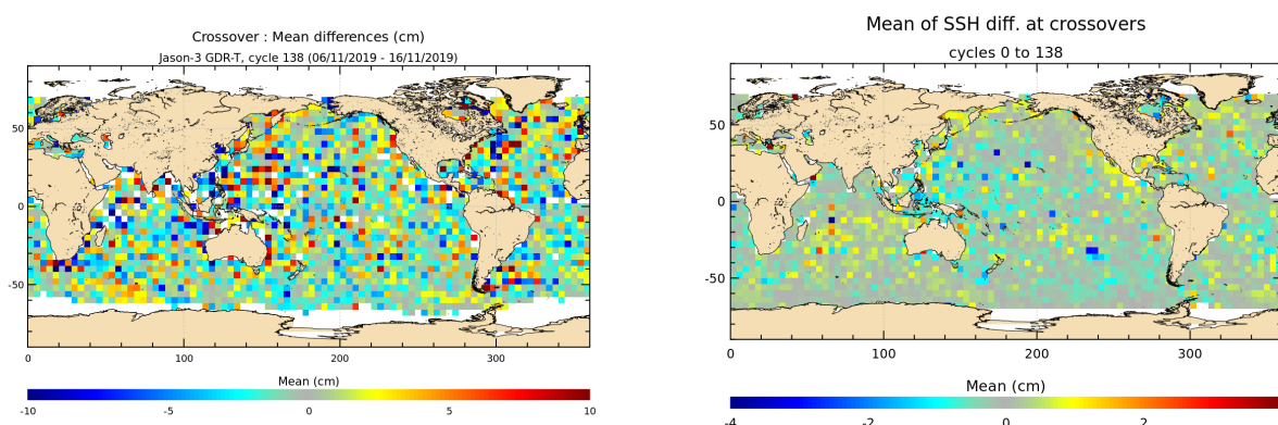
FIGURE 12 – Mean SSH at crossovers for cycle 138 (left) and over the whole Jason-3 period (right).
