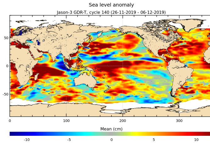
FIGURE 17 – Sea level anomaly relative to MSS for cycle 140.
