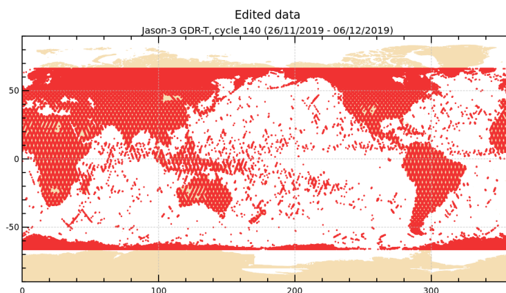
FIGURE 2 – Edited measurements for cycle 140.
