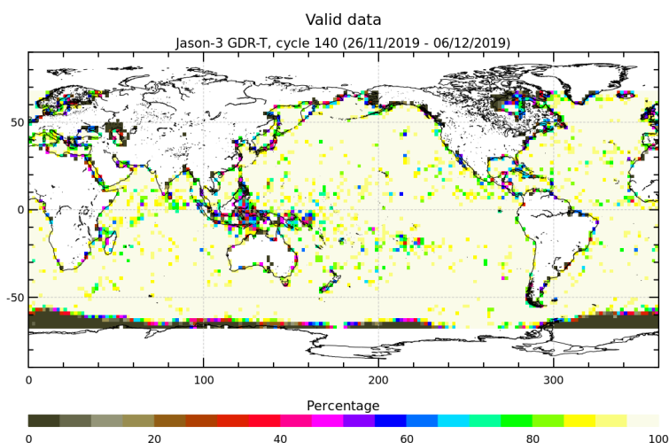
FIGURE 3 – Percentage of valid measurements for cycle 140.
