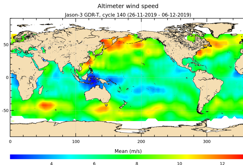
FIGURE 9 – Altimeter wind speed for cycle 140.
