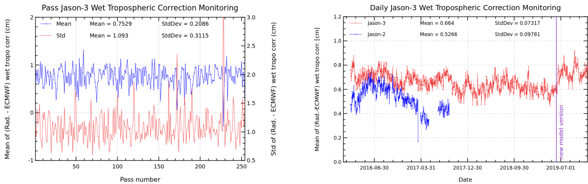
FIGURE 11 – Pass monitoring of wet troposphere differences between radiometer and ECMWF model for Jason-3 cycle 140 (left) and Jason-3 versus Jason-2 daily monitoring of wet troposphere differences between radiometer and ECMWF model (right).
