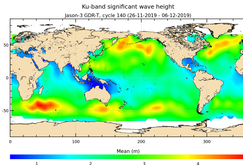
FIGURE 5 – Significant wave height for cycle 140.
