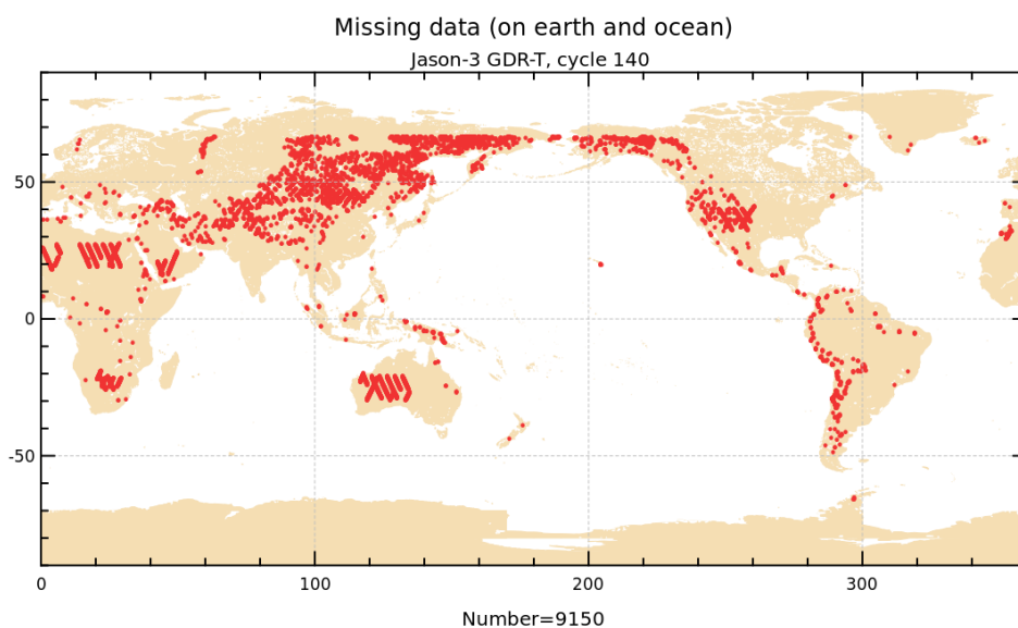
FIGURE 1 – Missing measurements for cycle 140.
