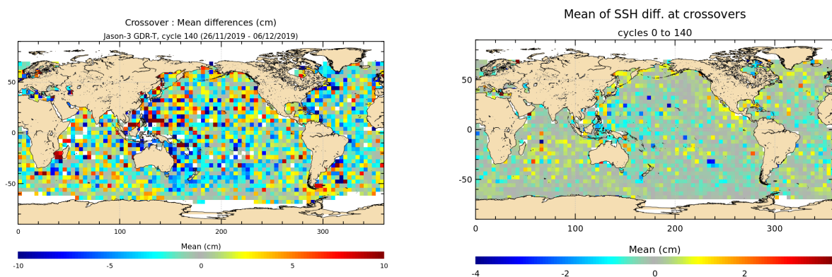
FIGURE 12 – Mean SSH at crossovers for cycle 140 (left) and over the whole Jason-3 period (right).
