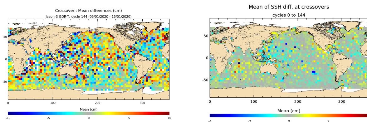
FIGURE 13 – Mean SSH at crossovers for cycle 144 (left) and over the whole Jason-3 period (right).
