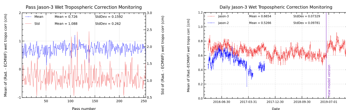
FIGURE 11 – Pass monitoring of wet troposphere differences between radiometer and ECMWF model for Jason-3 cycle 144 (left) and Jason-3 versus Jason-2 daily monitoring of wet troposphere differences between radiometer and ECMWF model (right).
