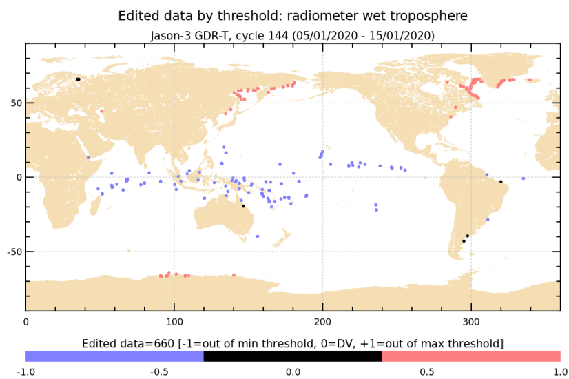
FIGURE 12 – Edited measurements by threshold for radiometer wet troposphere for cycle 144.
