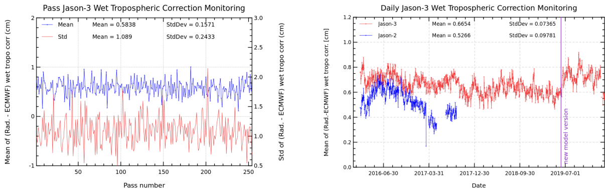
FIGURE 11 – Pass monitoring of wet troposphere differences between radiometer and ECMWF model for Jason-3 cycle 148 (left) and Jason-3 versus Jason-2 daily monitoring of wet troposphere differences between radiometer and ECMWF model (right).
