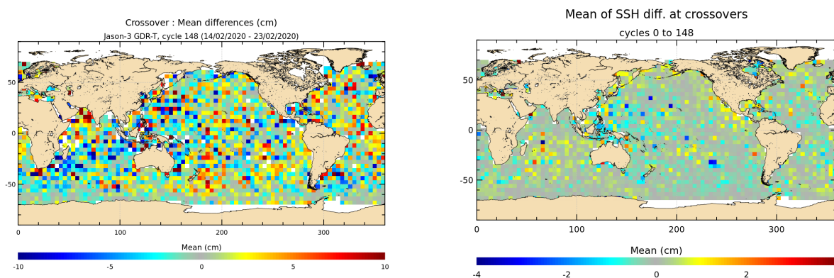
FIGURE 12 – Mean SSH at crossovers for cycle 148 (left) and over the whole Jason-3 period (right).
