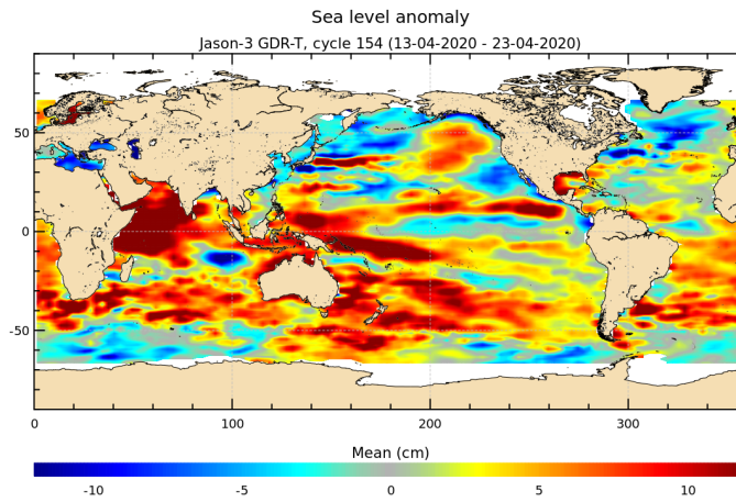
FIGURE 17 – Sea level anomaly relative to MSS for cycle 154.
