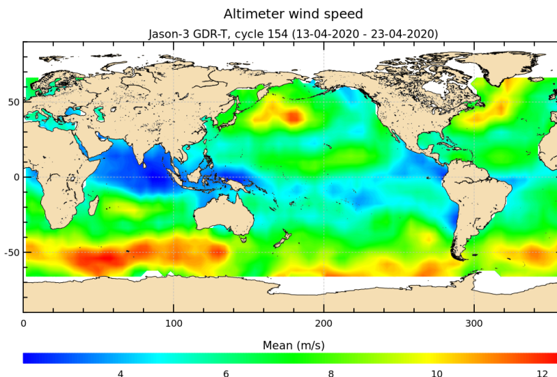
FIGURE 9 – Altimeter wind speed for cycle 154.
