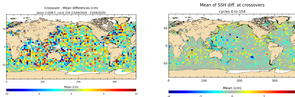
FIGURE 12 – Mean SSH at crossovers for cycle 154 (left) and over the whole Jason-3 period (right).
