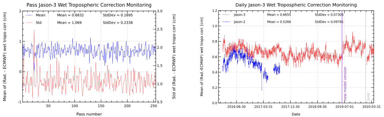
FIGURE 11 – Pass monitoring of wet troposphere differences between radiometer and ECMWF model for Jason-3 cycle 154 (left) and Jason-3 versus Jason-2 daily monitoring of wet troposphere differences between radiometer and ECMWF model (right).
