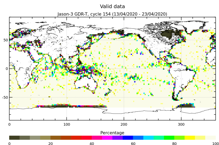
FIGURE 3 – Percentage of valid measurements for cycle 154.
