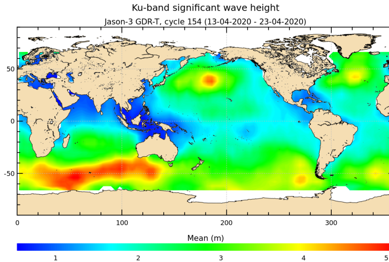
FIGURE 5 – Significant wave height for cycle 154.
