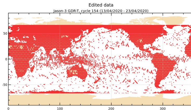
FIGURE 2 – Edited measurements for cycle 154.
