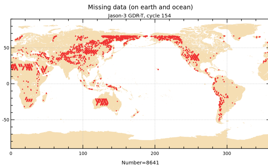
FIGURE 1 – Missing measurements for cycle 154.
