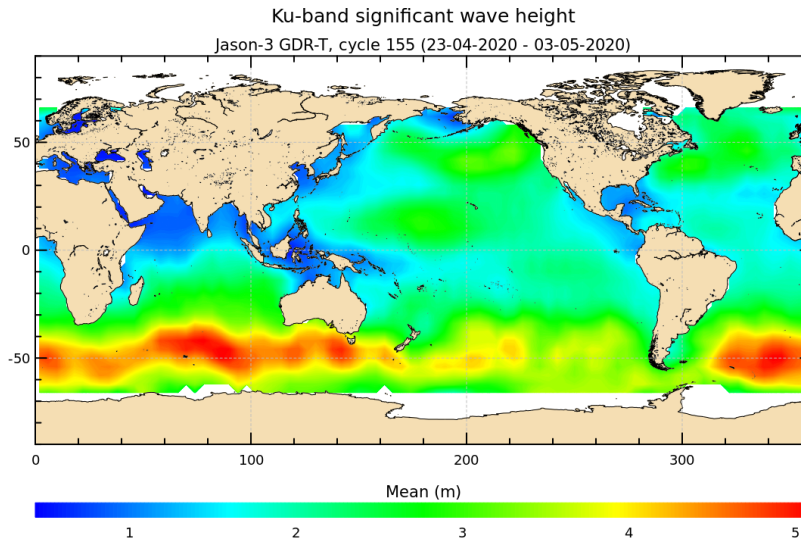
FIGURE 5 – Significant wave height for cycle 155.
