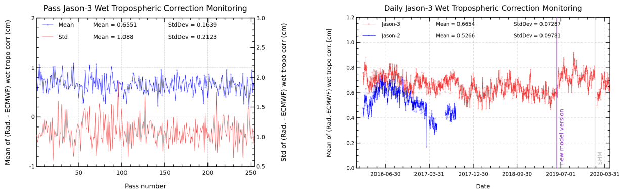
FIGURE 11 – Pass monitoring of wet troposphere differences between radiometer and ECMWF model for Jason-3 cycle 155 (left) and Jason-3 versus Jason-2 daily monitoring of wet troposphere differences between radiometer and ECMWF model (right).
