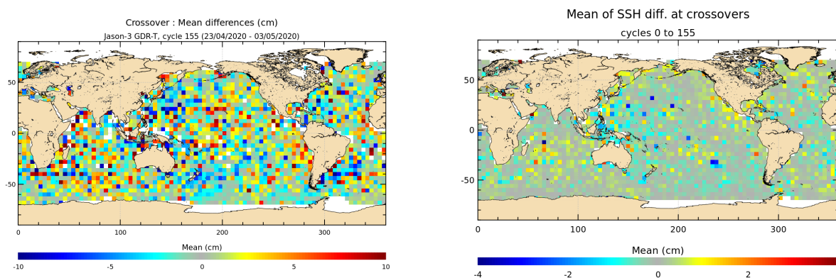
FIGURE 12 – Mean SSH at crossovers for cycle 155 (left) and over the whole Jason-3 period (right).
