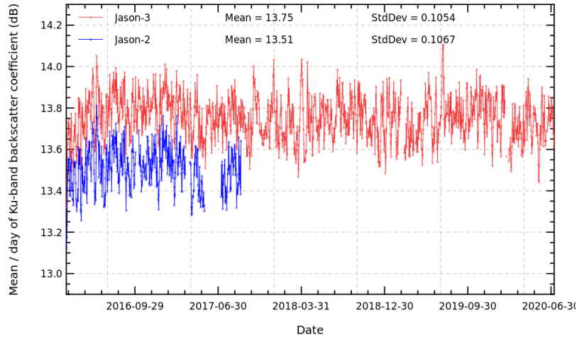
FIGURE 7 – Daily monitoring of Ku-band backscattering coefficient for Jason-2 and Jason-3.
