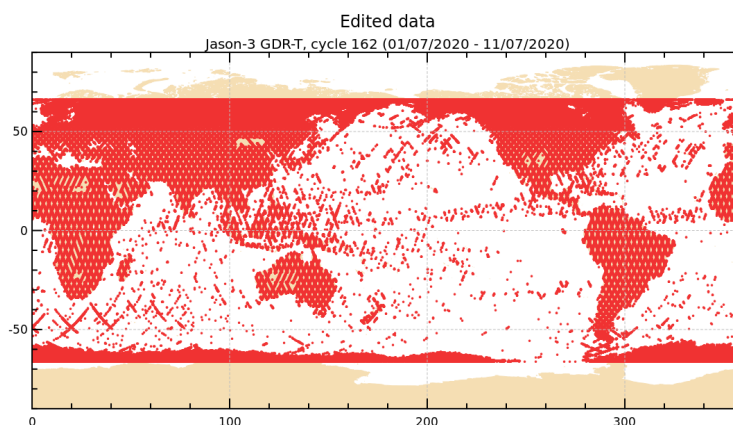
FIGURE 2 – Edited measurements for cycle 162.
