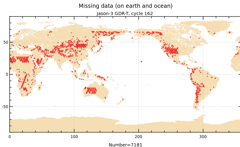
FIGURE 1 – Missing measurements for cycle 162.
