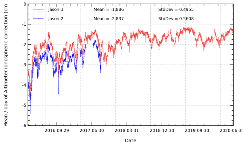
FIGURE 8 – Daily monitoring of dual-frequency ionosphere correction for Jason-2 and Jason-3.
