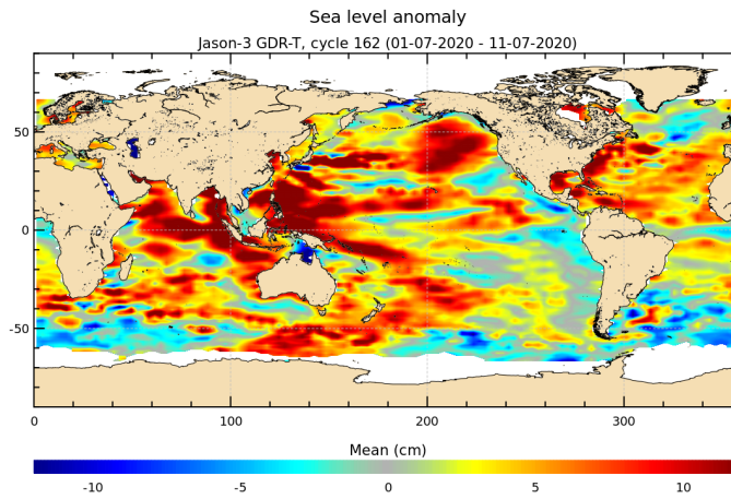
FIGURE 17 – Sea level anomaly relative to MSS for cycle 162.
