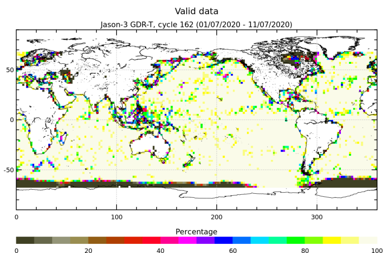
FIGURE 3 – Percentage of valid measurements for cycle 162.
