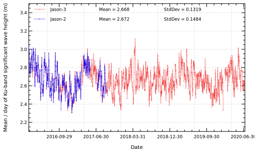
FIGURE 6 – Daily monitoring of Ku-band significant wave height for Jason-2 and Jason-3.
