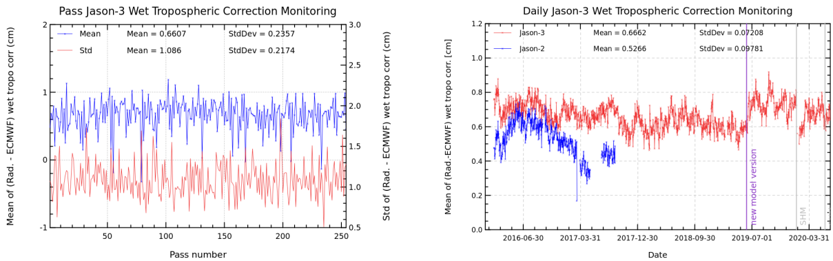
FIGURE 11 – Pass monitoring of wet troposphere differences between radiometer and ECMWF model for Jason-3 cycle 162 (left) and Jason-3 versus Jason-2 daily monitoring of wet troposphere differences between radiometer and ECMWF model (right).
