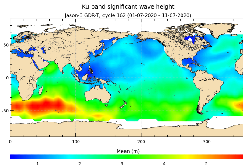
FIGURE 5 – Significant wave height for cycle 162.
