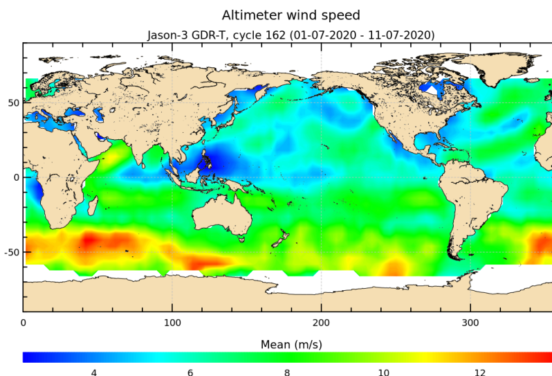
FIGURE 9 – Altimeter wind speed for cycle 162.
