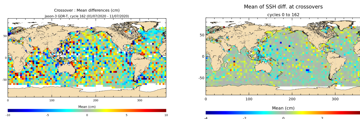
FIGURE 12 – Mean SSH at crossovers for cycle 162 (left) and over the whole Jason-3 period (right).
