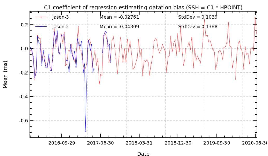
FIGURE 15 – Cyclic monitoring of pseudo time tag bias for Jason-3 and Jason-2.
