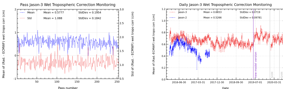
FIGURE 11 – Pass monitoring of wet troposphere differences between radiometer and ECMWF model for Jason-3 cycle 167 (left) and Jason-3 versus Jason-2 daily monitoring of wet troposphere differences between radiometer and ECMWF model (right).
