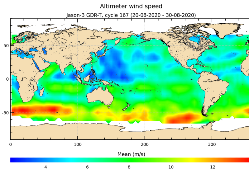
FIGURE 9 – Altimeter wind speed for cycle 167.
