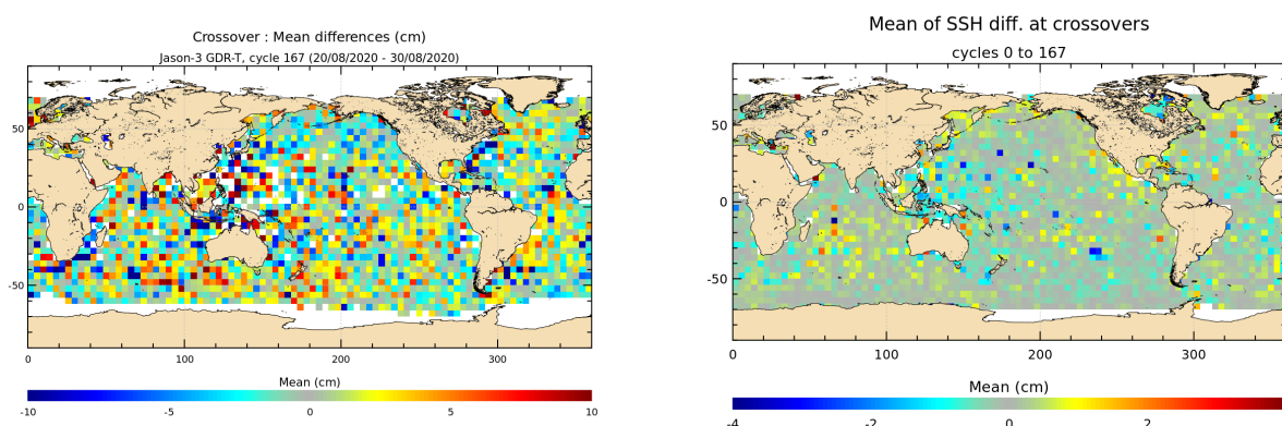
FIGURE 12 – Mean SSH at crossovers for cycle 167 (left) and over the whole Jason-3 period (right).
