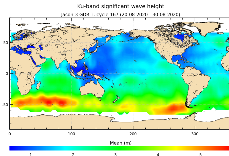
FIGURE 5 – Significant wave height for cycle 167.
