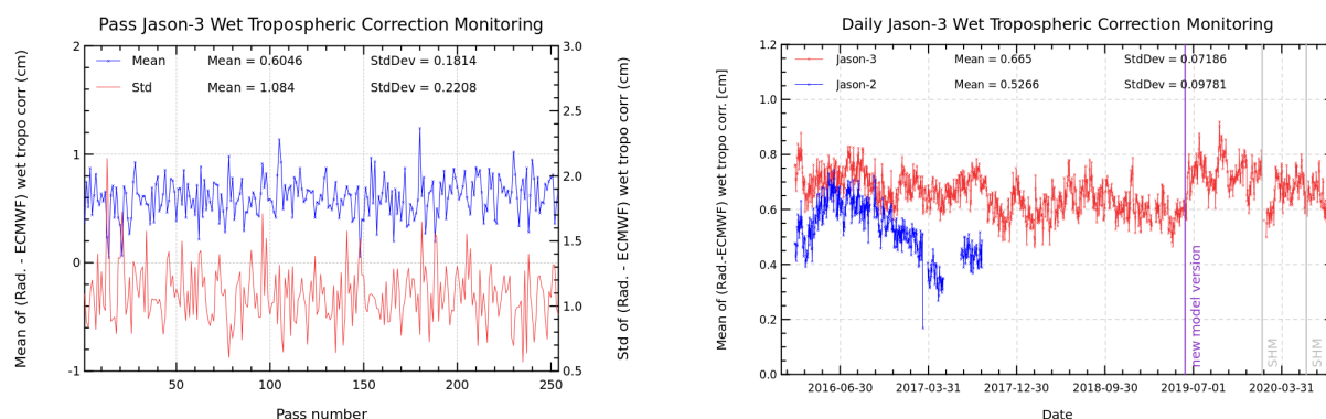
FIGURE 11 – Pass monitoring of wet troposphere differences between radiometer and ECMWF model for Jason-3 cycle 168 (left) and Jason-3 versus Jason-2 daily monitoring of wet troposphere differences between radiometer and ECMWF model (right).
