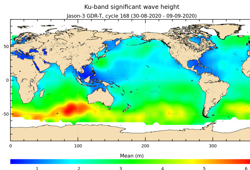
FIGURE 5 – Significant wave height for cycle 168.
