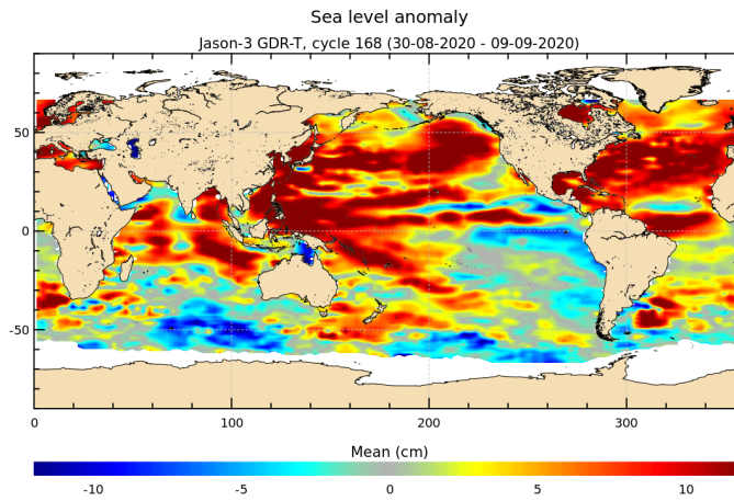
FIGURE 17 – Sea level anomaly relative to MSS for cycle 168.
