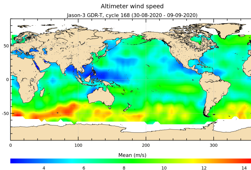
FIGURE 9 – Altimeter wind speed for cycle 168.
