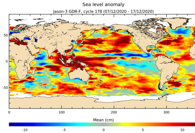
FIGURE 18 – Sea level anomaly relative to MSS for cycle 178.
