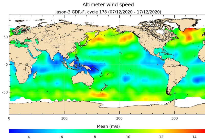
FIGURE 9 – Altimeter wind speed for cycle 178.
