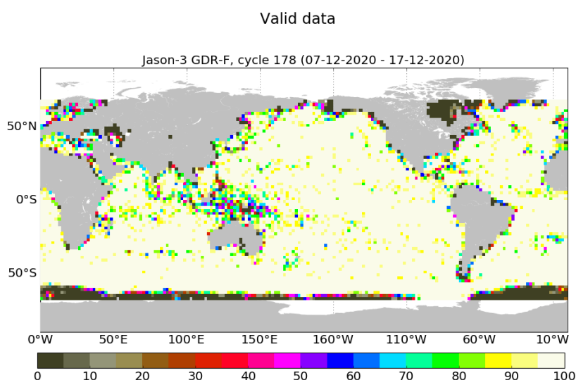
FIGURE 3 – Percentage of valid measurements for cycle 178.
