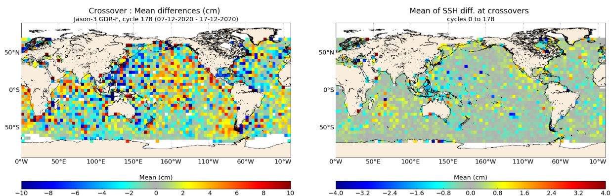
FIGURE 13 – Mean SSH at crossovers for cycle 178 (left) and over the whole Jason-3 period (right).
