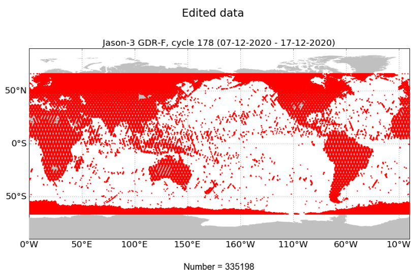
FIGURE 2 – Edited measurements for cycle 178.
