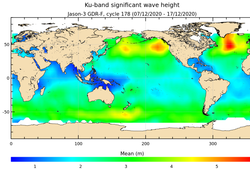
FIGURE 5 – Significant wave height for cycle 178.
