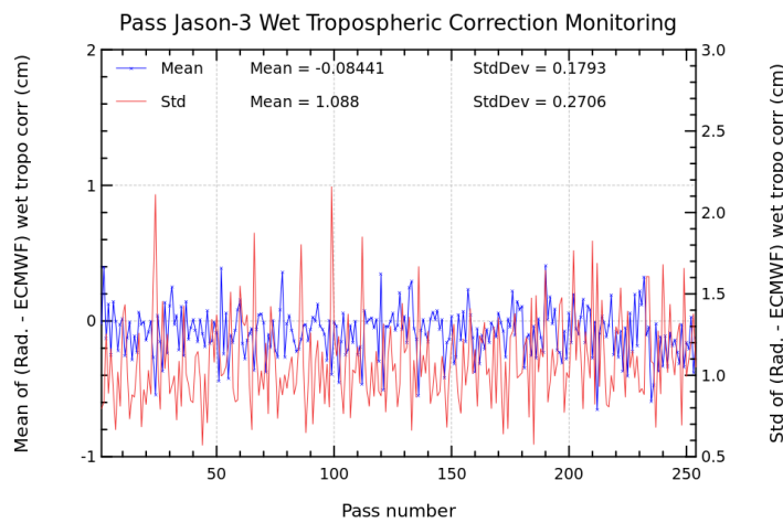
FIGURE 11 – Pass monitoring of wet troposphere differences between radiometer and ECMWF model for Jason-3 cycle 178
