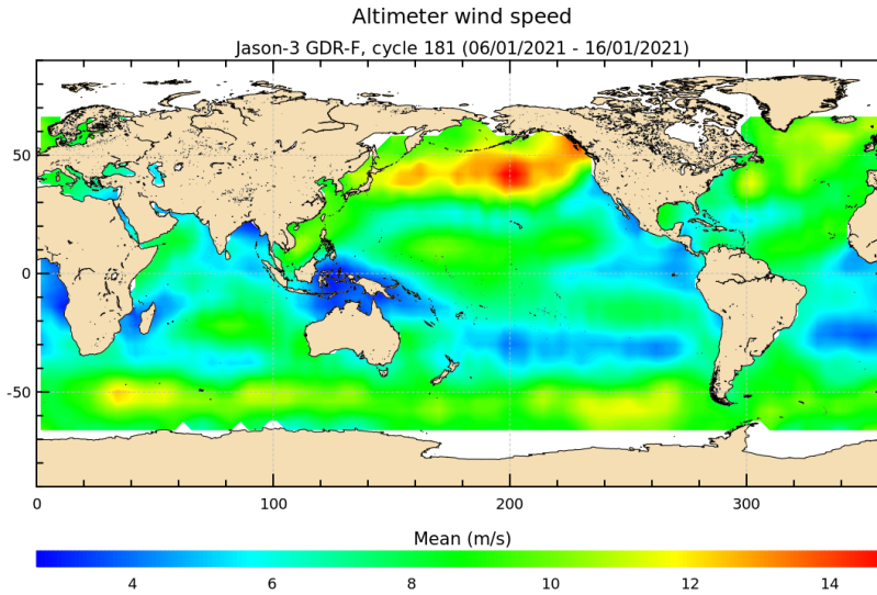
FIGURE 9 – Altimeter wind speed for cycle 181.
