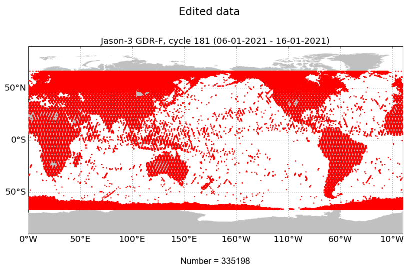
FIGURE 2 – Edited measurements for cycle 181.
