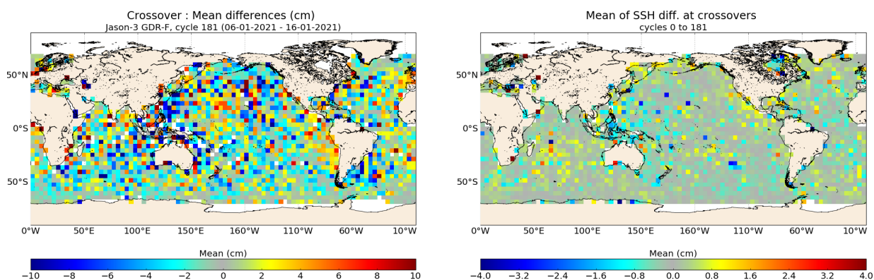
FIGURE 13 – Mean SSH at crossovers for cycle 181 (left) and over the whole Jason-3 period (right).
