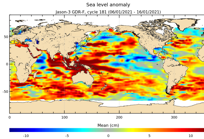
FIGURE 18 – Sea level anomaly relative to MSS for cycle 181.
