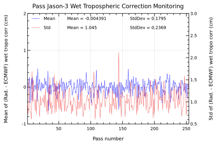
FIGURE 11 – Pass monitoring of wet troposphere differences between radiometer and ECMWF model for Jason-3 cycle 181
