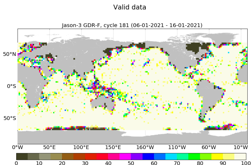
FIGURE 3 – Percentage of valid measurements for cycle 181.
