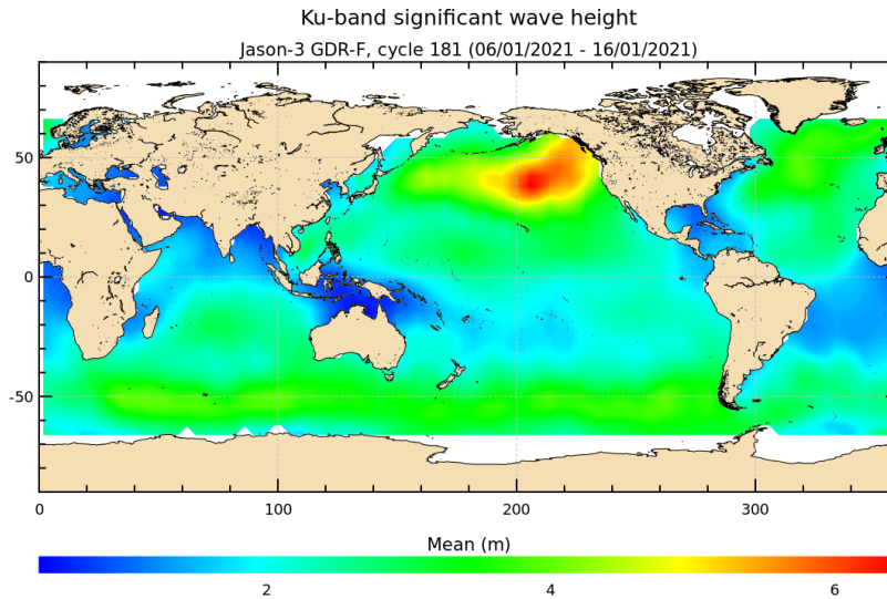
FIGURE 5 – Significant wave height for cycle 181.
