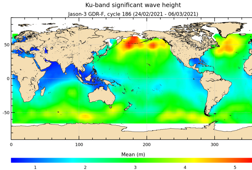
FIGURE 5 – Significant wave height for cycle 186.
