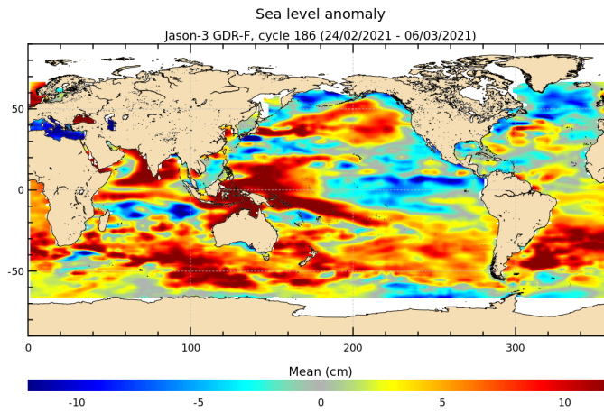
FIGURE 18 – Sea level anomaly relative to MSS for cycle 186.
