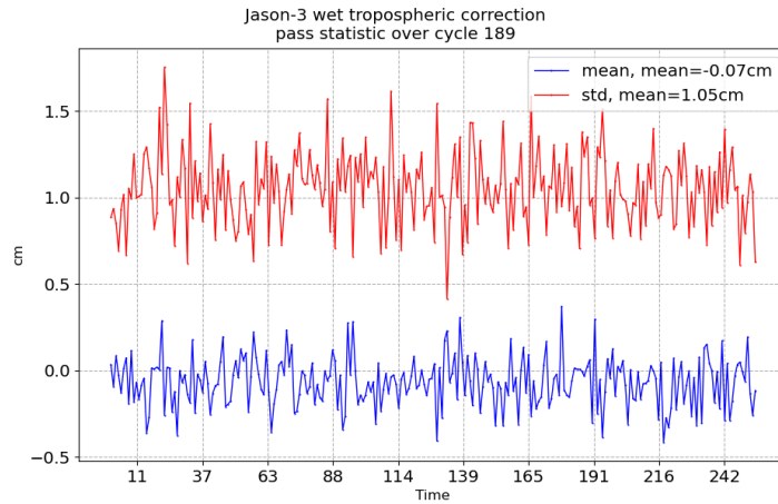
FIGURE 11 – Pass monitoring of wet troposphere differences between radiometer and ECMWF model for Jason-3 cycle 189
