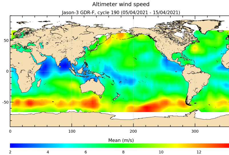
FIGURE 9 – Altimeter wind speed for cycle 190.
