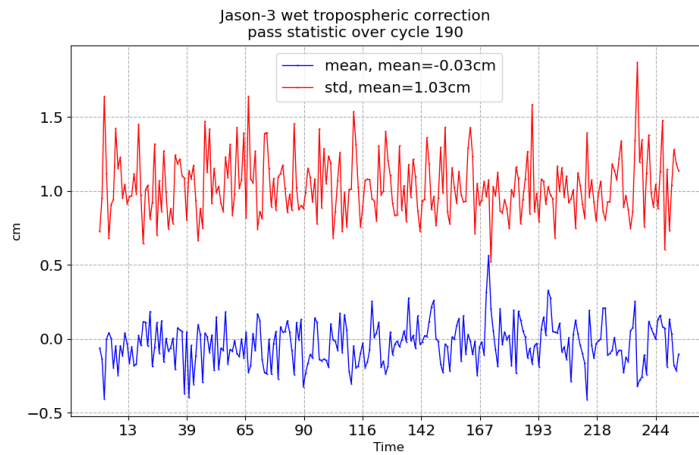
FIGURE 11 – Pass monitoring of wet troposphere differences between radiometer and ECMWF model for Jason-3 cycle 190
