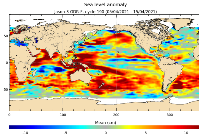
FIGURE 18 – Sea level anomaly relative to MSS for cycle 190.
