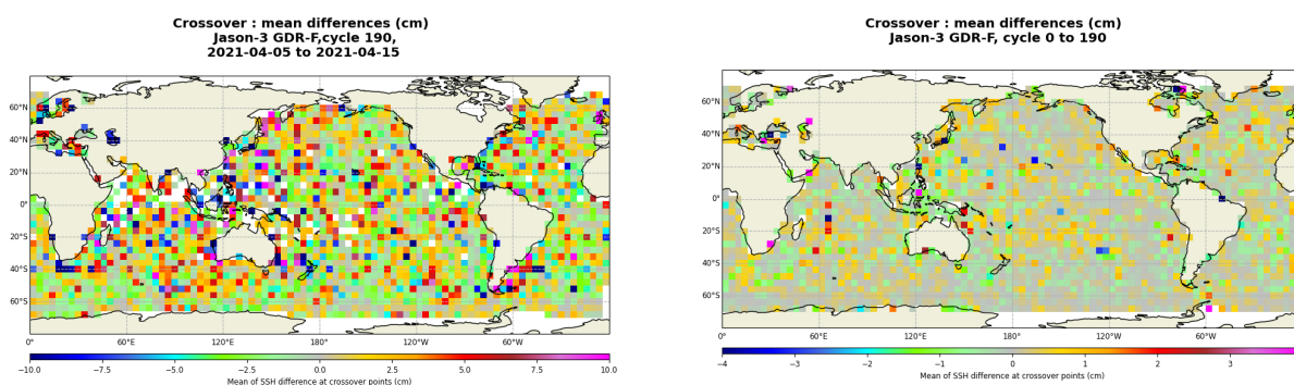
FIGURE 13 – Mean SSH at crossovers for cycle 190 (left) and over the whole Jason-3 period (right).
