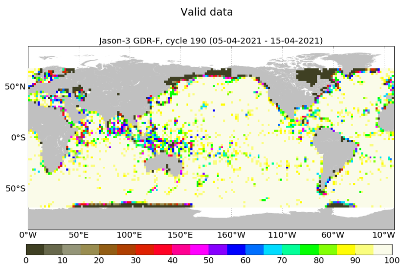
FIGURE 3 – Percentage of valid measurements for cycle 190.
