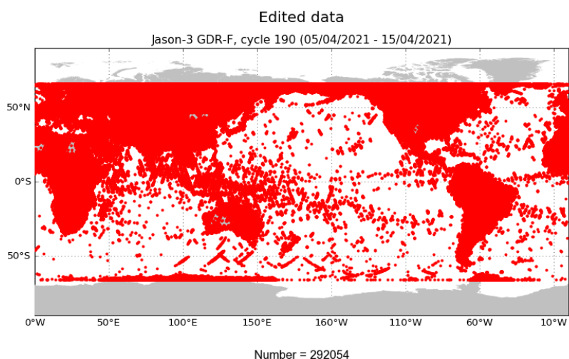
FIGURE 2 – Edited measurements for cycle 190.
