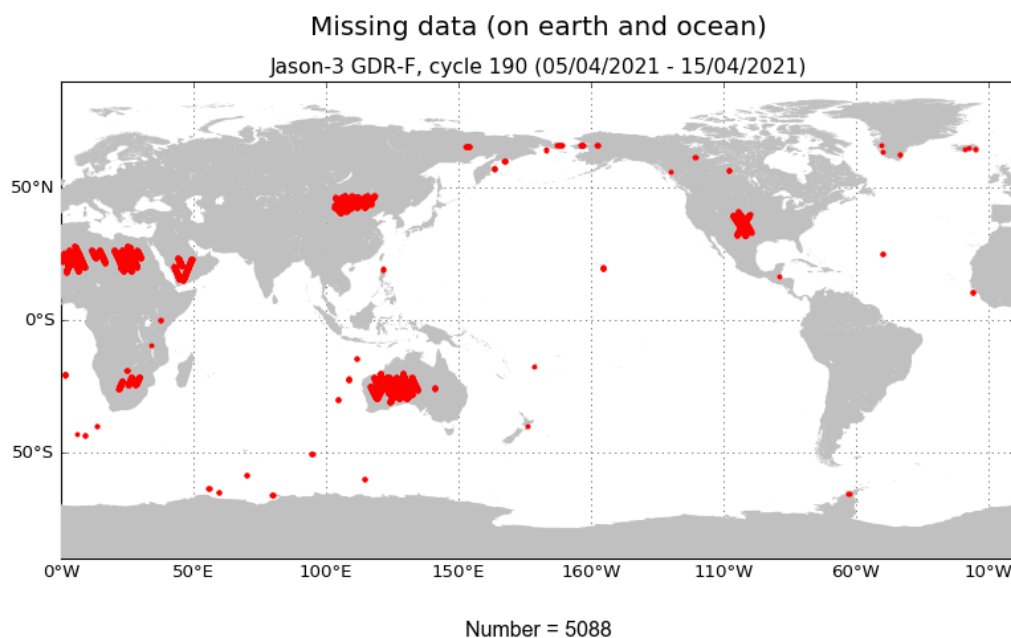
FIGURE 1 – Missing measurements for cycle 190.
