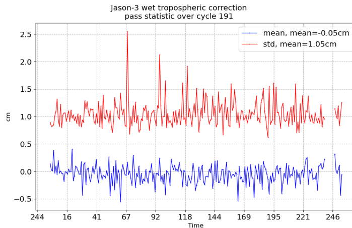
FIGURE 11 – Pass monitoring of wet troposphere differences between radiometer and ECMWF model for Jason-3 cycle 191
