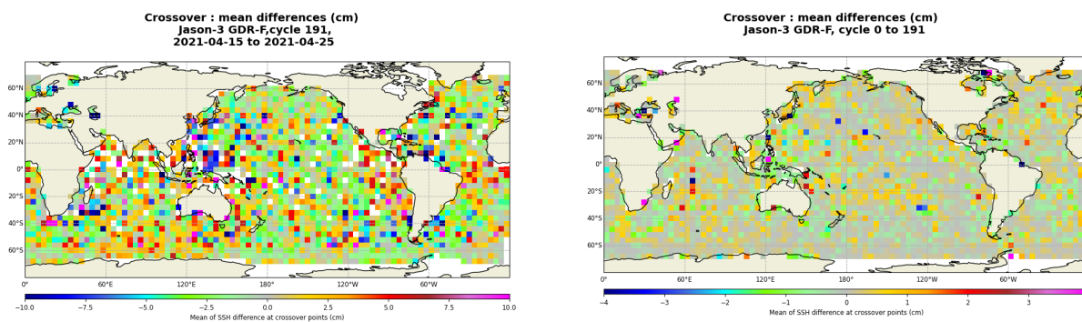
FIGURE 13 – Mean SSH at crossovers for cycle 191 (left) and over the whole Jason-3 period (right).
