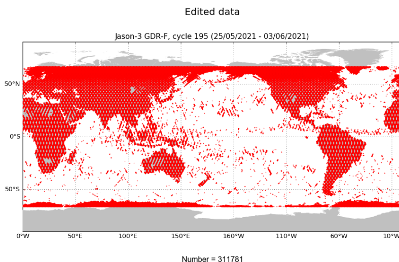
FIGURE 2 – Edited measurements for cycle 195.
