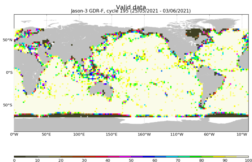
FIGURE 3 – Percentage of valid measurements for cycle 195.
