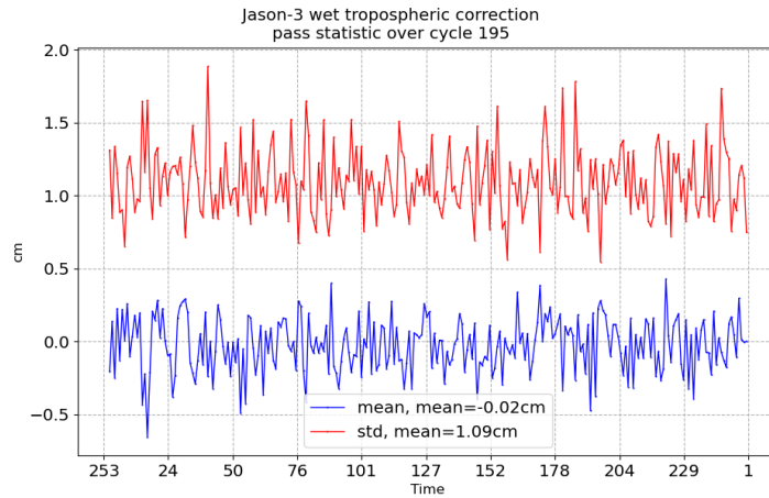
FIGURE 11 – Pass monitoring of wet troposphere differences between radiometer and ECMWF model for Jason-3 cycle 195
