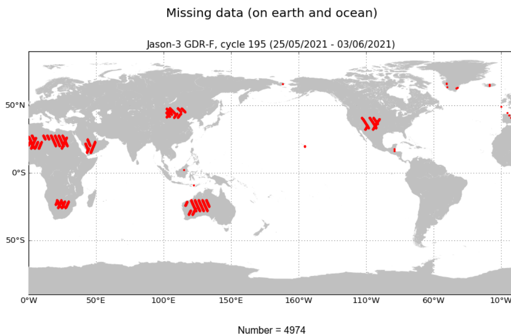
FIGURE 1 – Missing measurements for cycle 195.
