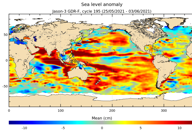
FIGURE 18 – Sea level anomaly relative to MSS for cycle 195.
