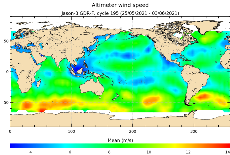
FIGURE 9 – Altimeter wind speed for cycle 195.
