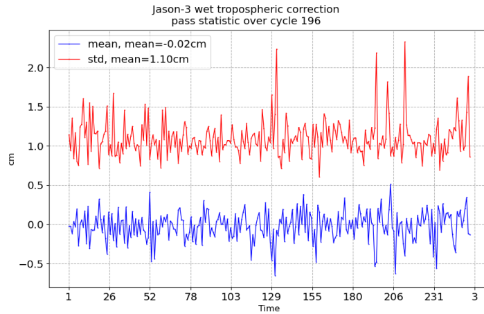
FIGURE 11 – Pass monitoring of wet troposphere differences between radiometer and ECMWF model for Jason-3 cycle 196
