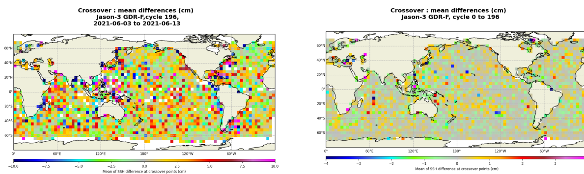
FIGURE 13 – Mean SSH at crossovers for cycle 196 (left) and over the whole Jason-3 period (right).
