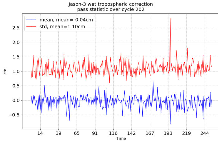
FIGURE 11 – Pass monitoring of wet troposphere differences between radiometer and ECMWF model for Jason-3 cycle 202
