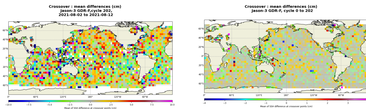
FIGURE 13 – Mean SSH at crossovers for cycle 202 (left) and over the whole Jason-3 period (right).
