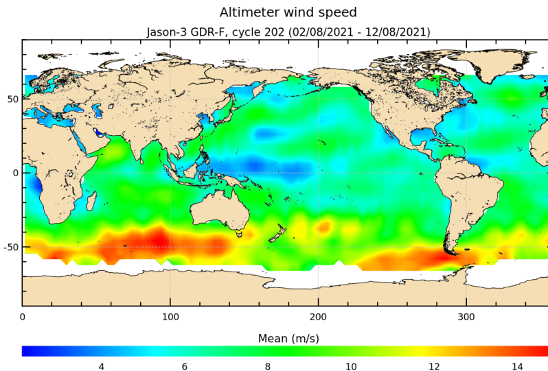
FIGURE 9 – Altimeter wind speed for cycle 202.
