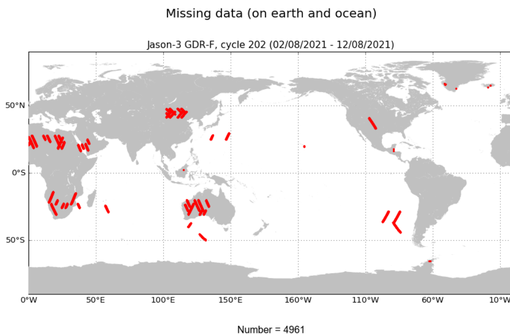
FIGURE 1 – Missing measurements for cycle 202.
