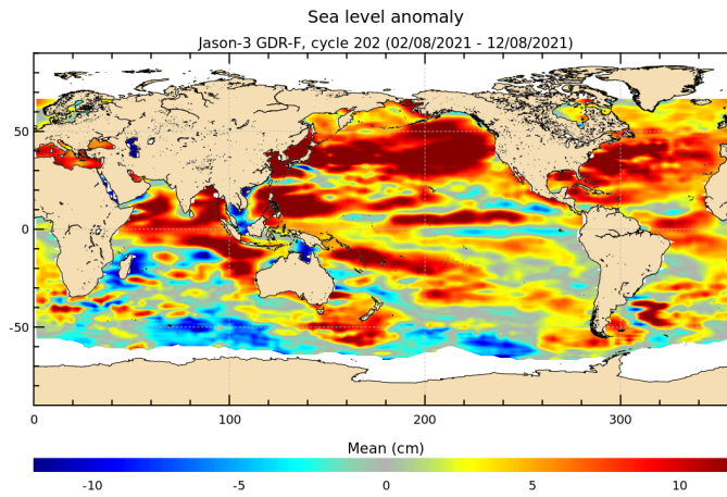
FIGURE 18 – Sea level anomaly relative to MSS for cycle 202.
