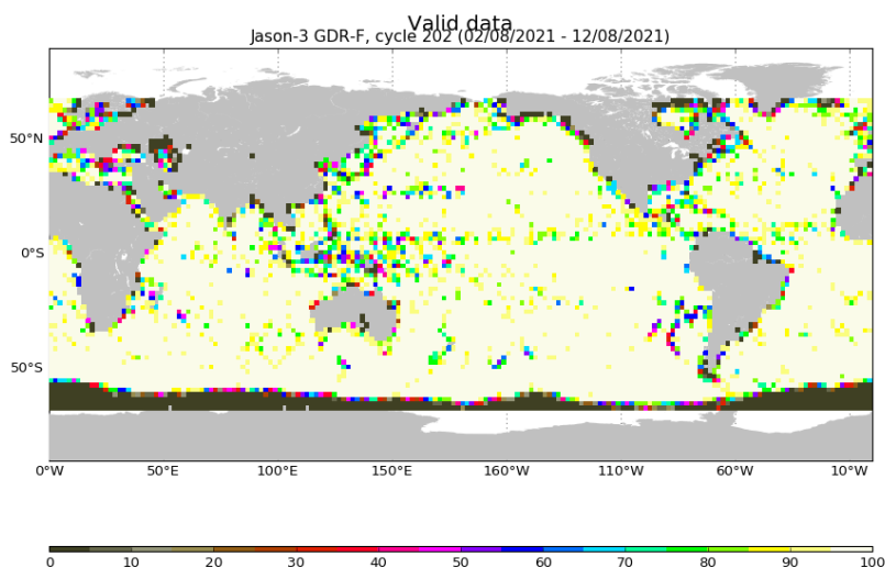
FIGURE 3 – Percentage of valid measurements for cycle 202.
