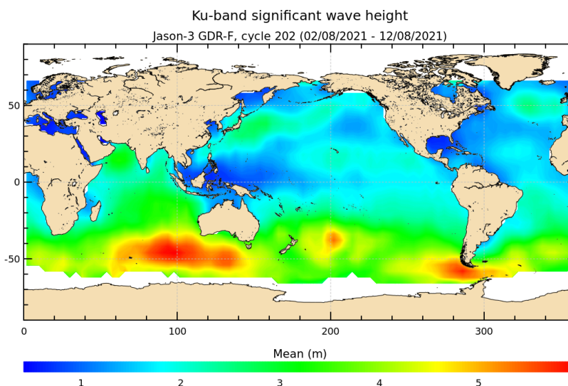
FIGURE 5 – Significant wave height for cycle 202.
