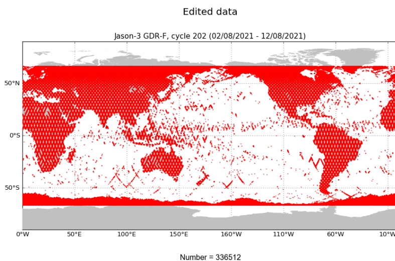
FIGURE 2 – Edited measurements for cycle 202.
