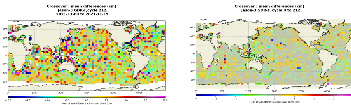
FIGURE 13 – Mean SSH at crossovers for cycle 212 (left) and over the whole Jason-3 period (right).
