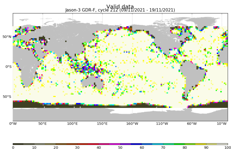
FIGURE 3 – Percentage of valid measurements for cycle 212.
