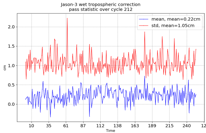
FIGURE 11 – Pass monitoring of wet troposphere differences between radiometer and ECMWF model for Jason-3 cycle 212
