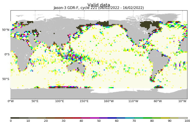
FIGURE 3 – Percentage of valid measurements for cycle 221.
