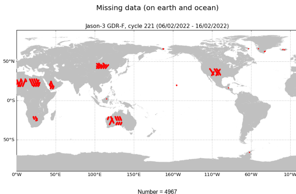
FIGURE 1 – Missing measurements for cycle 221.
