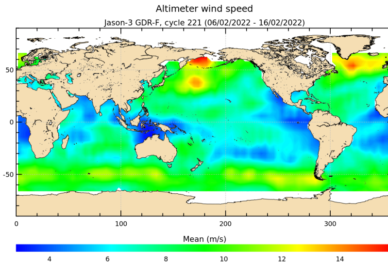
FIGURE 9 – Altimeter wind speed for cycle 221.
