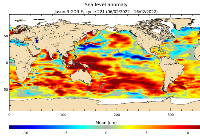
FIGURE 18 – Sea level anomaly relative to MSS for cycle 221.
