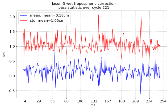
FIGURE 11 – Pass monitoring of wet troposphere differences between radiometer and ECMWF model for Jason-3 cycle 221
