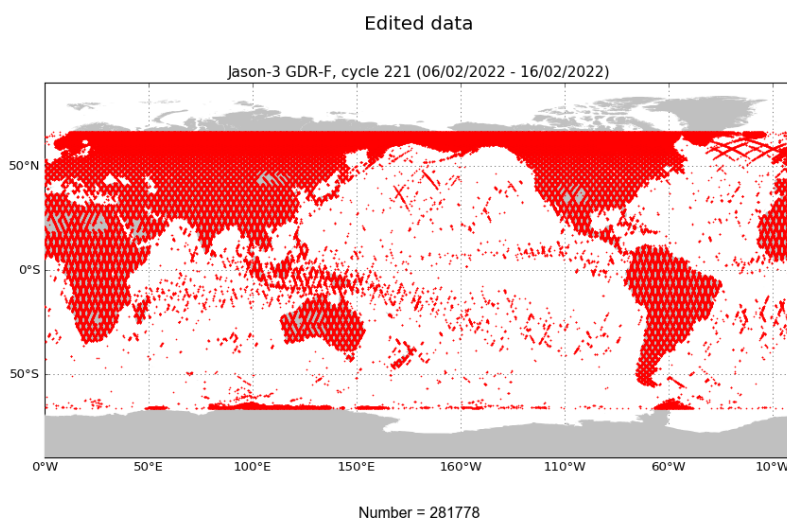
FIGURE 2 – Edited measurements for cycle 221.
