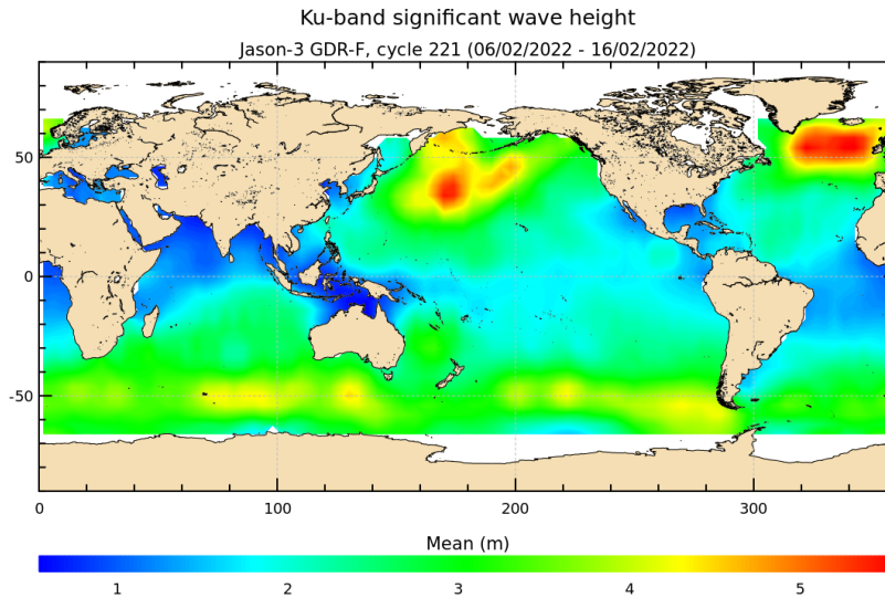
FIGURE 5 – Significant wave height for cycle 221.
