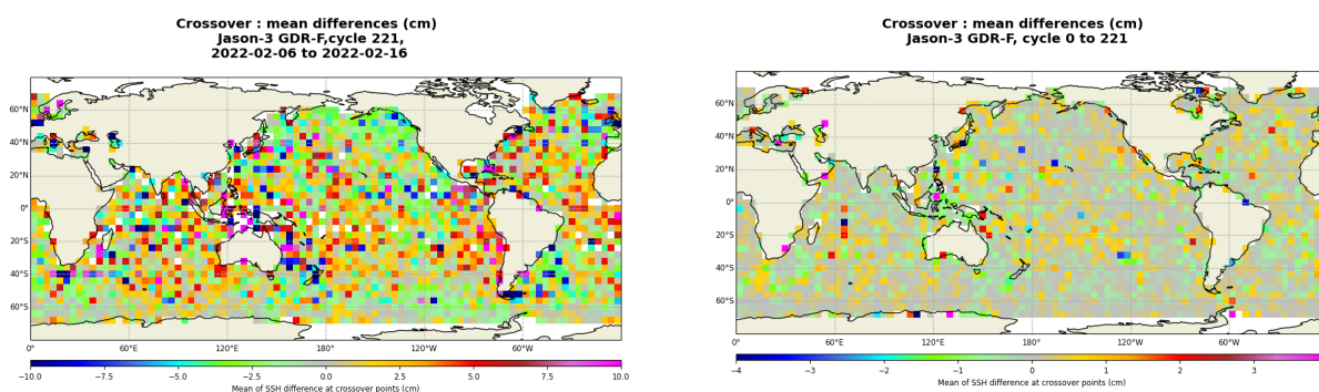
FIGURE 13 – Mean SSH at crossovers for cycle 221 (left) and over the whole Jason-3 period (right).
