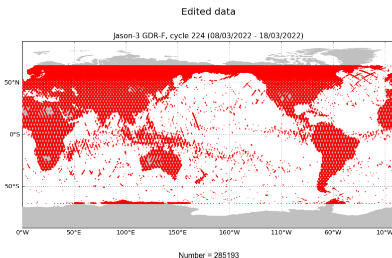
FIGURE 2 – Edited measurements for cycle 224.
