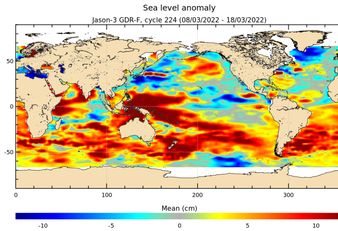
FIGURE 18 – Sea level anomaly relative to MSS for cycle 224.
