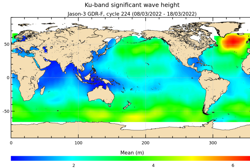
FIGURE 5 – Significant wave height for cycle 224.
