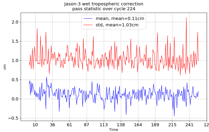
FIGURE 11 – Pass monitoring of wet troposphere differences between radiometer and ECMWF model for Jason-3 cycle 224
