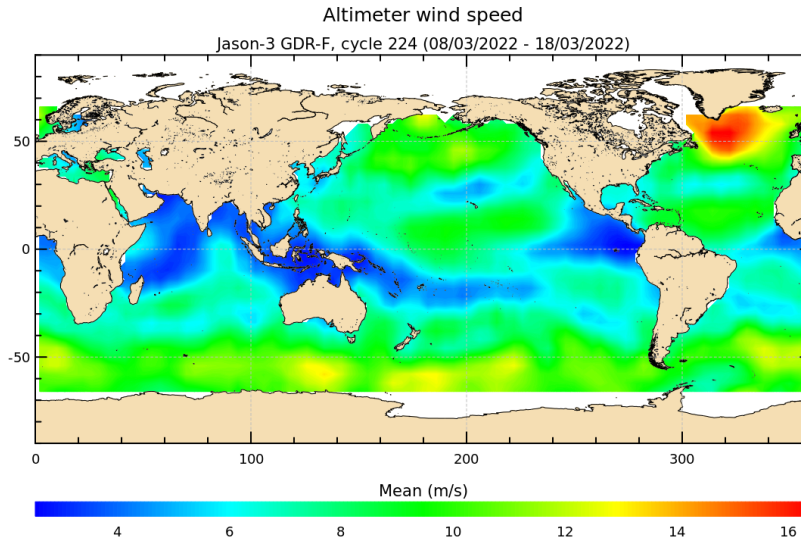
FIGURE 9 – Altimeter wind speed for cycle 224.
