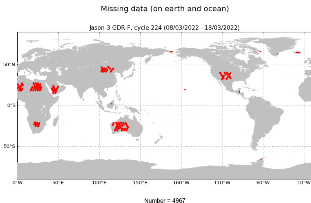
FIGURE 1 – Missing measurements for cycle 224.
