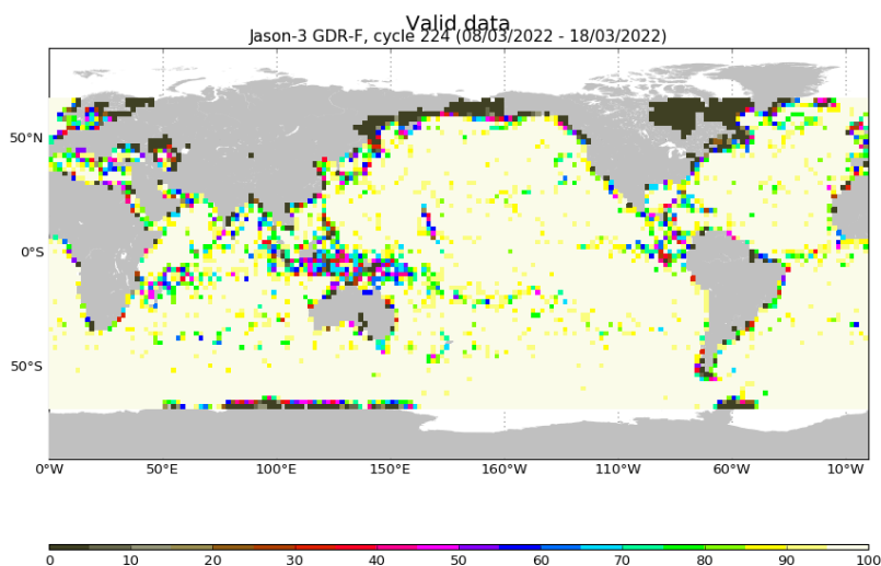
FIGURE 3 – Percentage of valid measurements for cycle 224.
