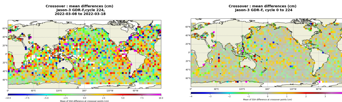
FIGURE 13 – Mean SSH at crossovers for cycle 224 (left) and over the whole Jason-3 period (right).
