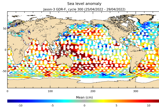
FIGURE 18 – Sea level anomaly relative to MSS for cycle 300.
