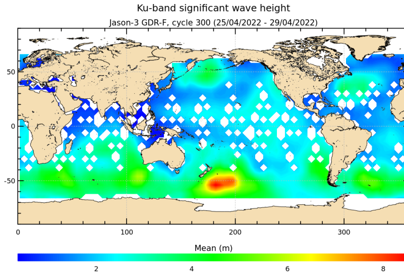
FIGURE 5 – Significant wave height for cycle 300.
