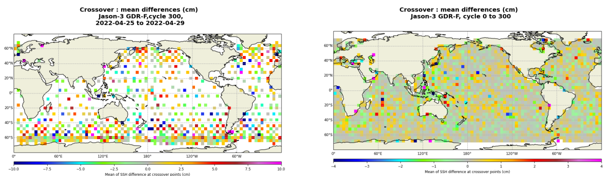
FIGURE 13 – Mean SSH at crossovers for cycle 300 (left) and over the whole Jason-3 period (right).
