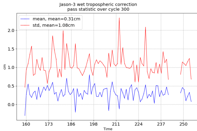
FIGURE 11 – Pass monitoring of wet troposphere differences between radiometer and ECMWF model for Jason-3 cycle 300
