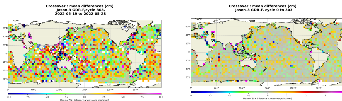
FIGURE 13 – Mean SSH at crossovers for cycle 303 (left) and over the whole Jason-3 period (right).
