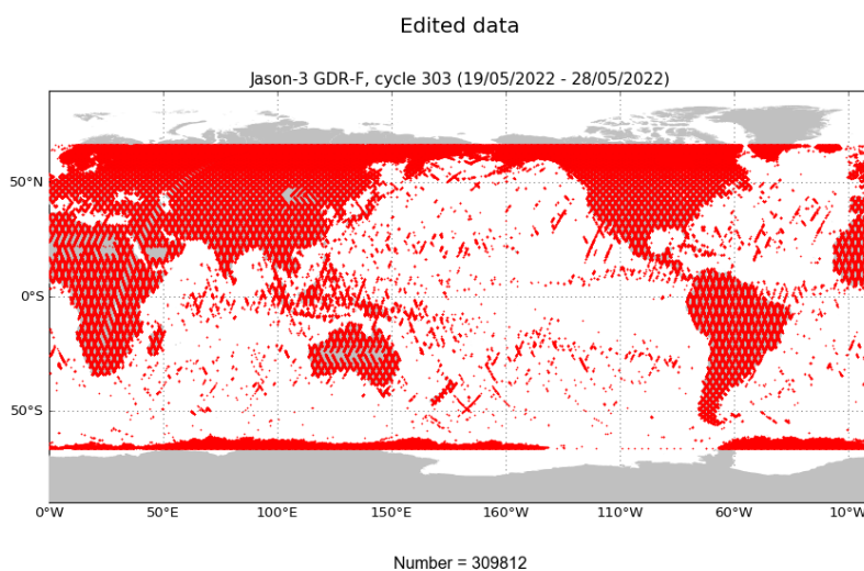
FIGURE 2 – Edited measurements for cycle 303.
