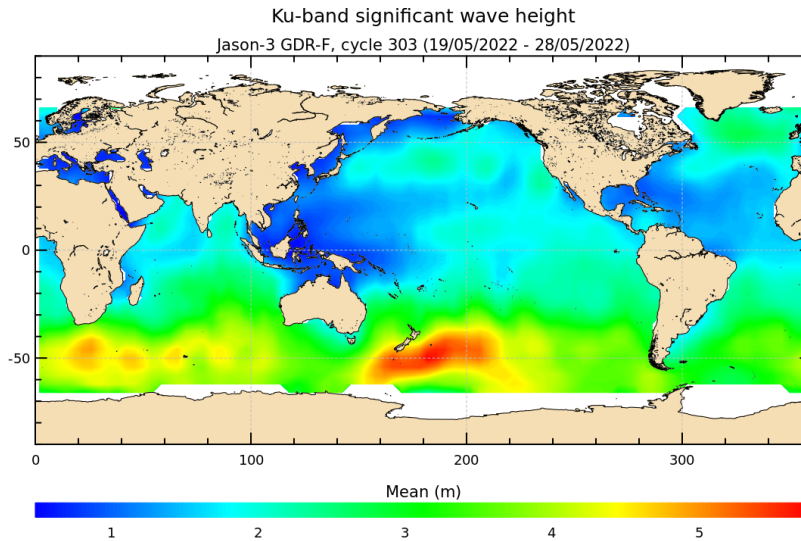
FIGURE 5 – Significant wave height for cycle 303.
