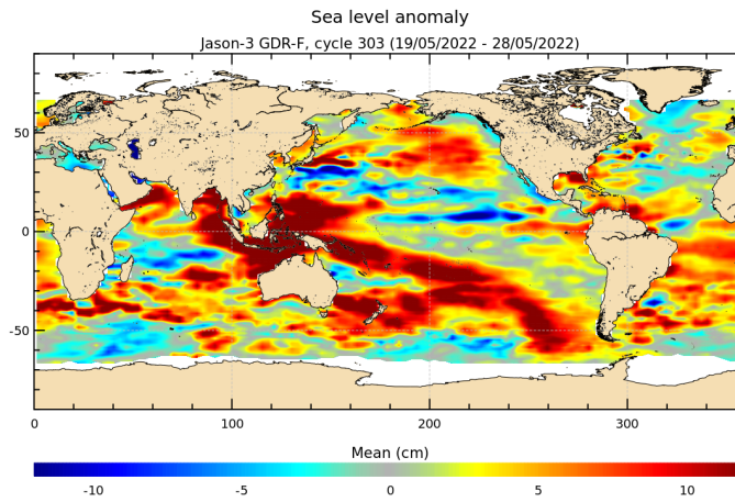
FIGURE 18 – Sea level anomaly relative to MSS for cycle 303.
