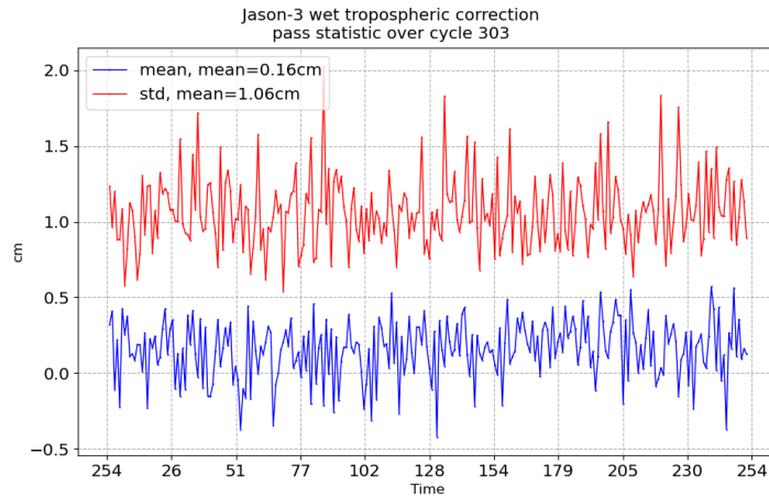
FIGURE 11 – Pass monitoring of wet troposphere differences between radiometer and ECMWF model for Jason-3 cycle 303
