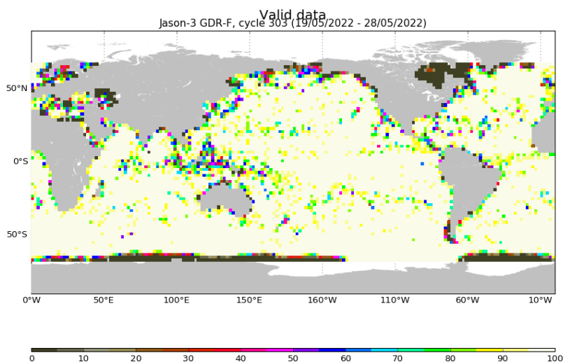
FIGURE 3 – Percentage of valid measurements for cycle 303.
