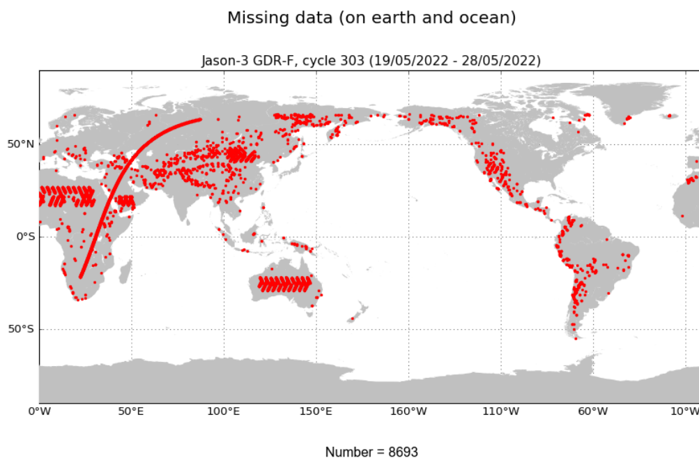
FIGURE 1 – Missing measurements for cycle 303.
