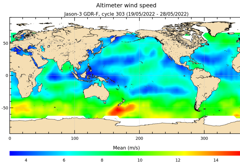
FIGURE 9 – Altimeter wind speed for cycle 303.
