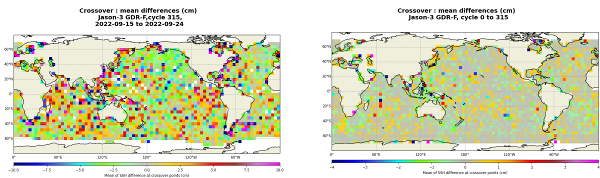
FIGURE 13 – Mean SSH at crossovers for cycle 315 (left) and over the whole Jason-3 period (right).
