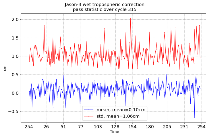
FIGURE 11 – Pass monitoring of wet troposphere differences between radiometer and ECMWF model for Jason-3 cycle 315
