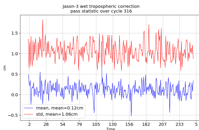
FIGURE 11 – Pass monitoring of wet troposphere differences between radiometer and ECMWF model for Jason-3 cycle 316
