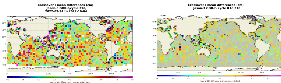
FIGURE 13 – Mean SSH at crossovers for cycle 316 (left) and over the whole Jason-3 period (right).
