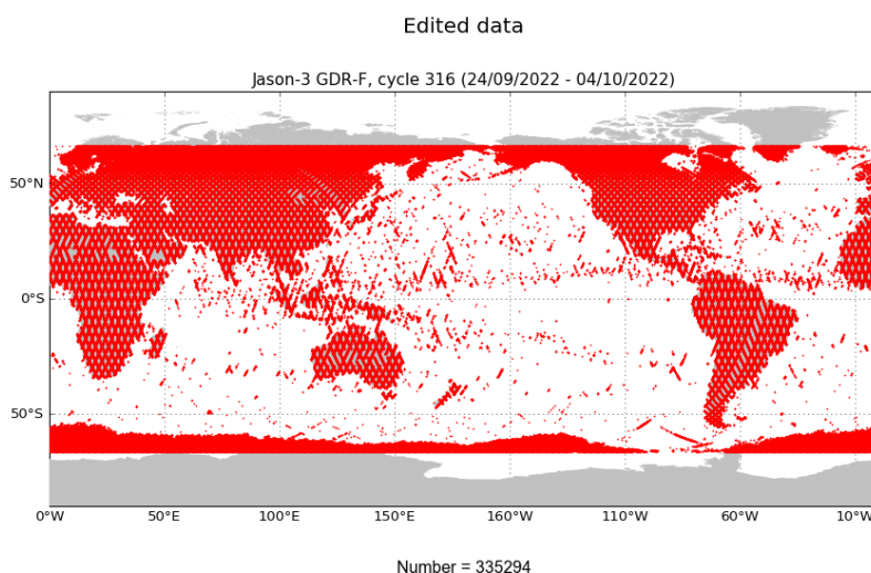
FIGURE 2 – Edited measurements for cycle 316.
