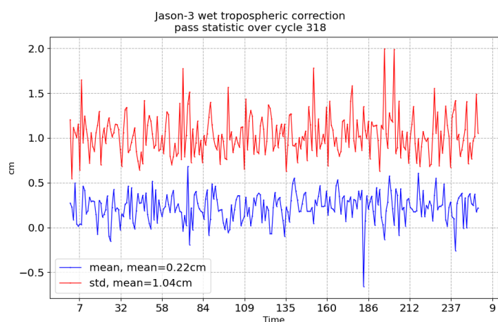
FIGURE 11 – Pass monitoring of wet troposphere differences between radiometer and ECMWF model for Jason-3 cycle 318
