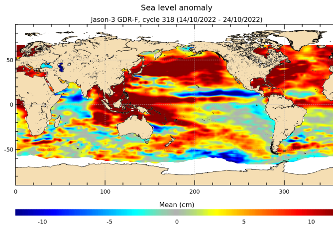
FIGURE 18 – Sea level anomaly relative to MSS for cycle 318.
