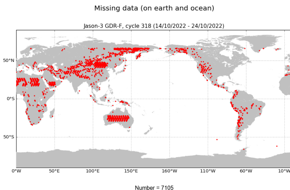
FIGURE 1 – Missing measurements for cycle 318.
