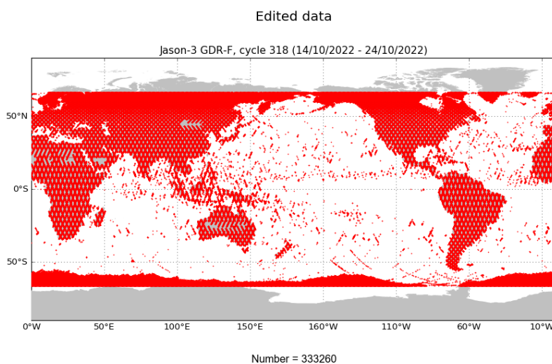
FIGURE 2 – Edited measurements for cycle 318.
