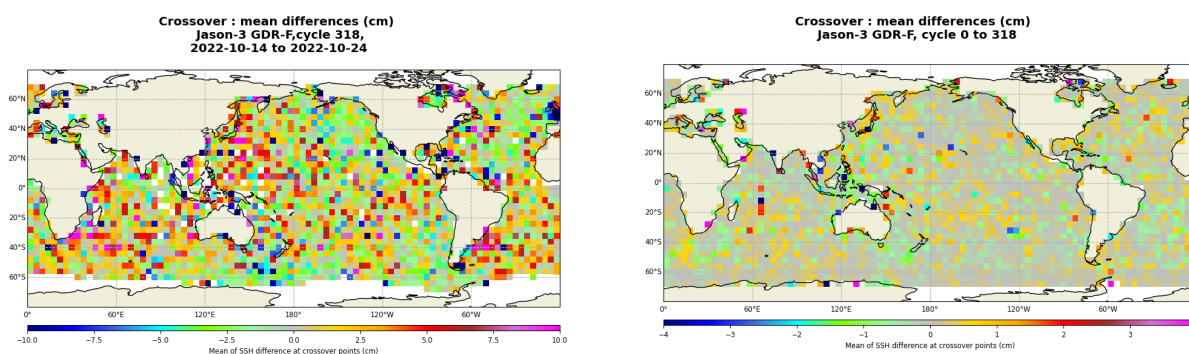
FIGURE 13 – Mean SSH at crossovers for cycle 318 (left) and over the whole Jason-3 period (right).
