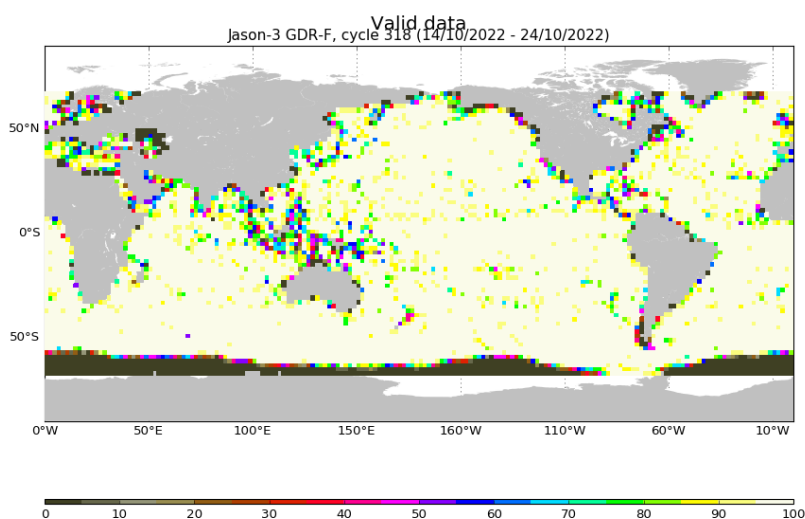
FIGURE 3 – Percentage of valid measurements for cycle 318.
