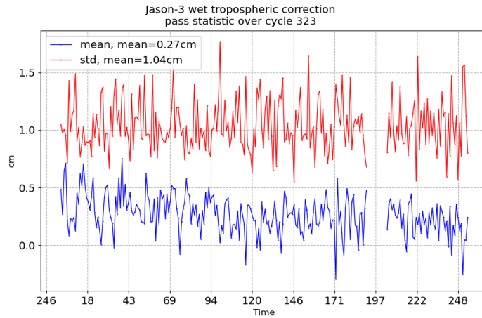
FIGURE 11 – Pass monitoring of wet troposphere differences between radiometer and ECMWF model for Jason-3 cycle 323
