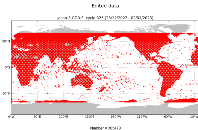
FIGURE 2 – Edited measurements for cycle 325.
