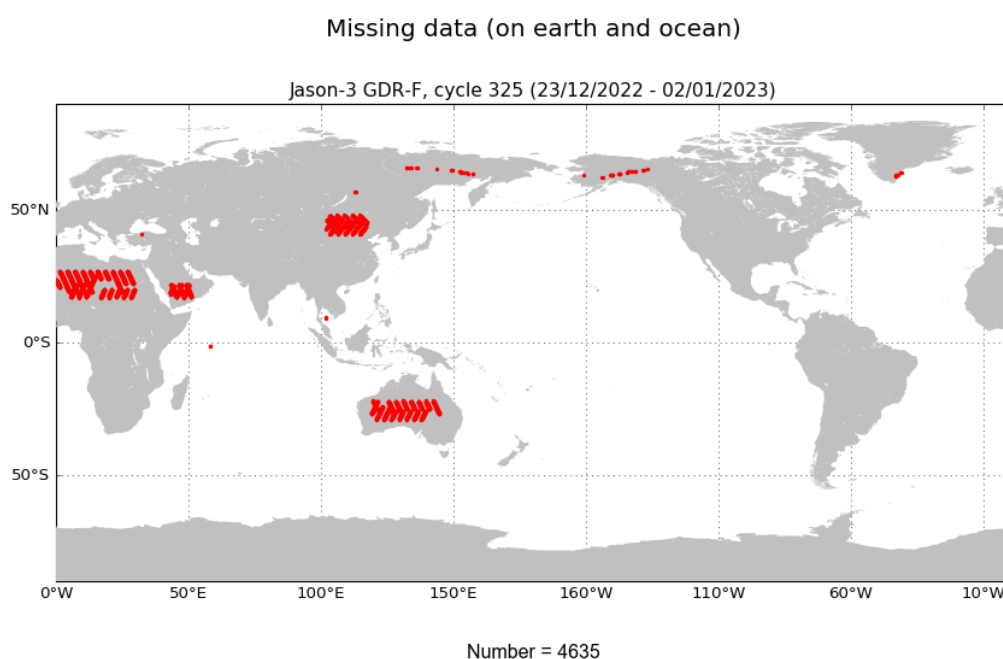
FIGURE 1 – Missing measurements for cycle 325.
