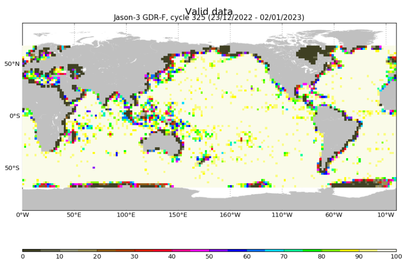
FIGURE 3 – Percentage of valid measurements for cycle 325.
