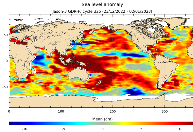
FIGURE 18 – Sea level anomaly relative to MSS for cycle 325.
