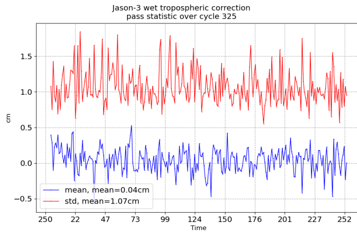
FIGURE 11 – Pass monitoring of wet troposphere differences between radiometer and ECMWF model for Jason-3 cycle 325
