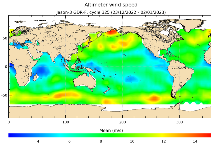
FIGURE 9 – Altimeter wind speed for cycle 325.
