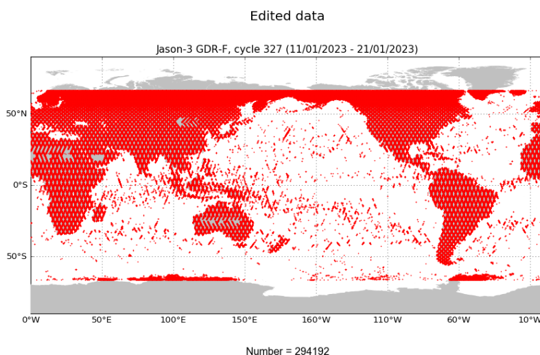
FIGURE 2 – Edited measurements for cycle 327.
