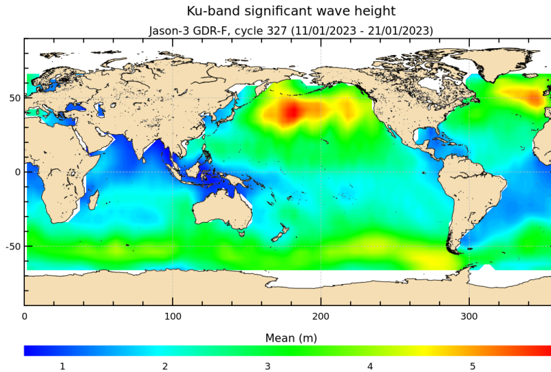
FIGURE 5 – Significant wave height for cycle 327.
