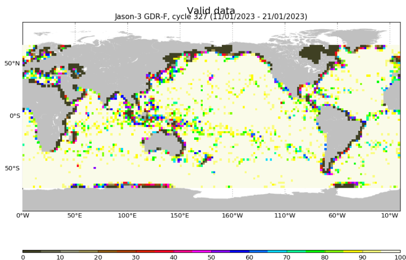
FIGURE 3 – Percentage of valid measurements for cycle 327.
