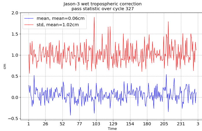
FIGURE 11 – Pass monitoring of wet troposphere differences between radiometer and ECMWF model for Jason-3 cycle 327
