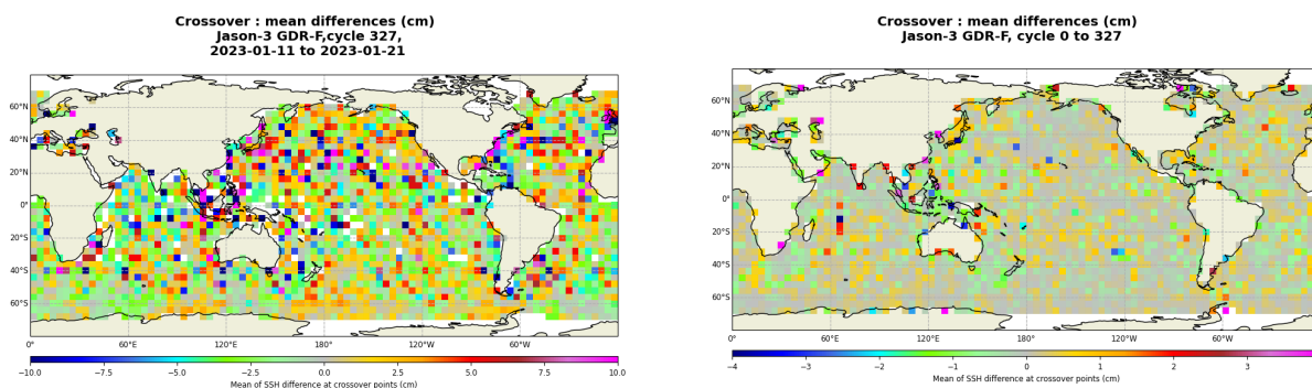
FIGURE 13 – Mean SSH at crossovers for cycle 327 (left) and over the whole Jason-3 period (right).
