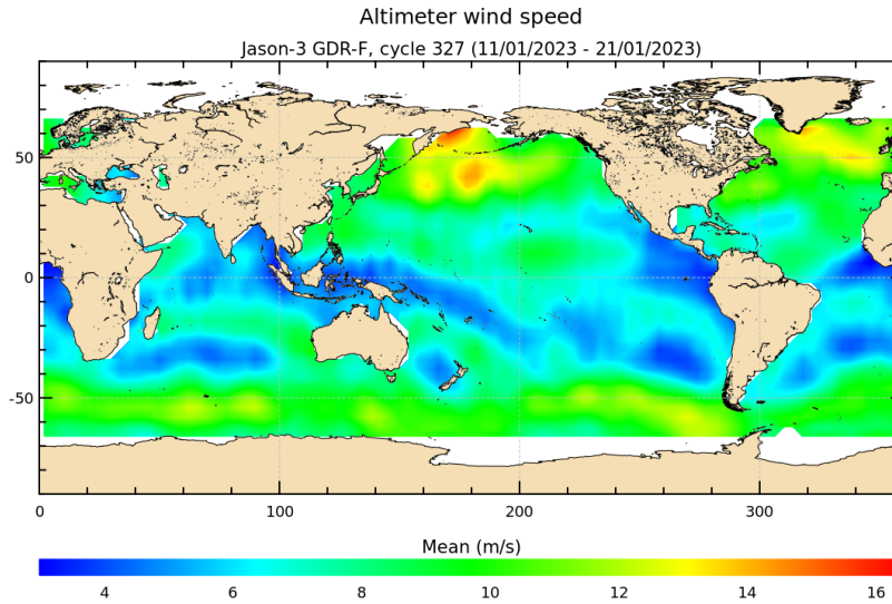
FIGURE 9 – Altimeter wind speed for cycle 327.
