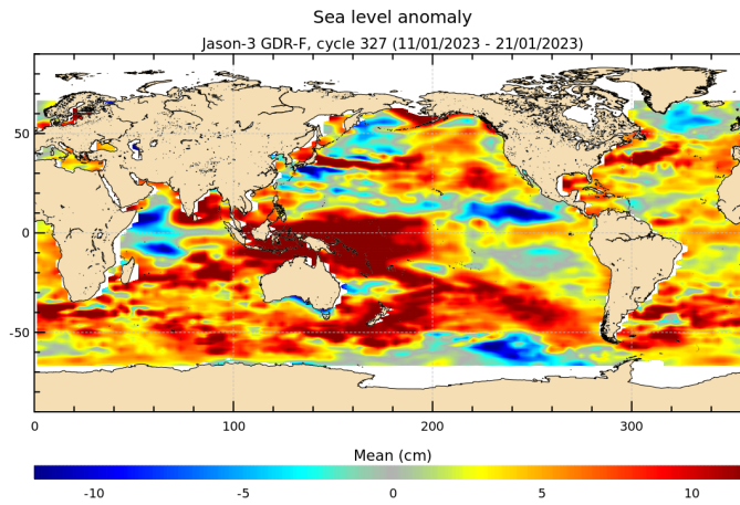
FIGURE 18 – Sea level anomaly relative to MSS for cycle 327.
