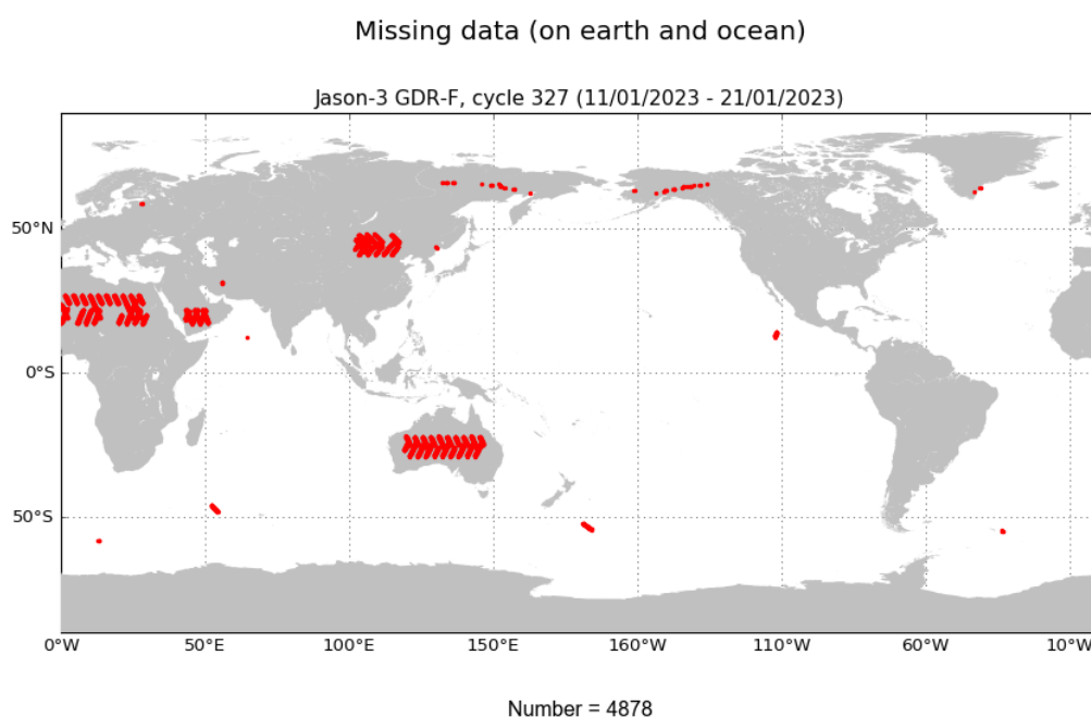
FIGURE 1 – Missing measurements for cycle 327.
