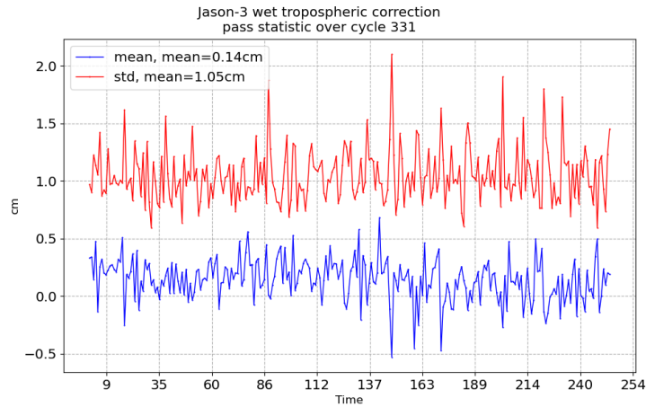
FIGURE 11 – Pass monitoring of wet troposphere differences between radiometer and ECMWF model for Jason-3 cycle 331
