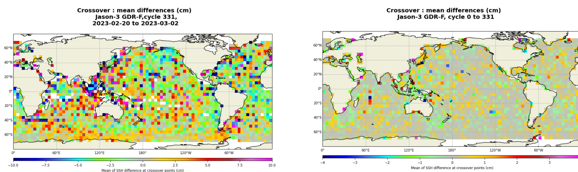
FIGURE 13 – Mean SSH at crossovers for cycle 331 (left) and over the whole Jason-3 period (right).
