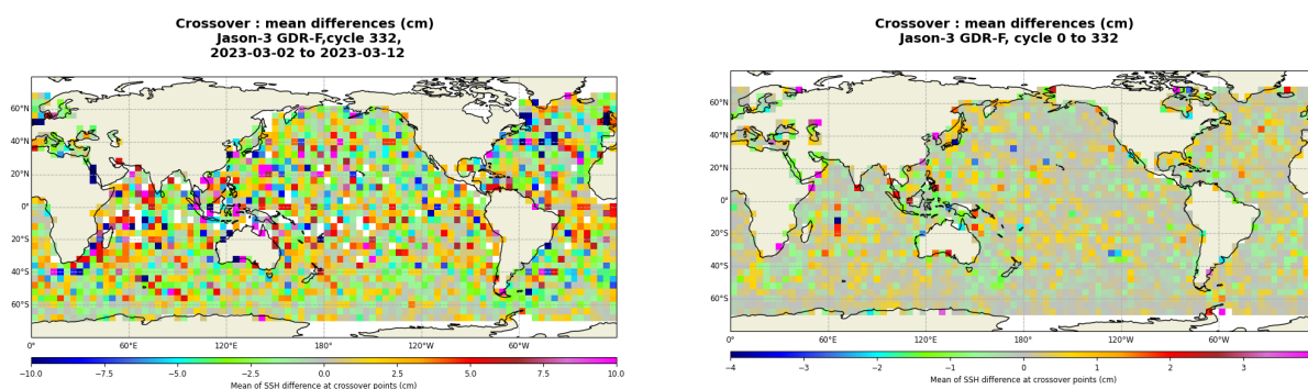
FIGURE 13 – Mean SSH at crossovers for cycle 332 (left) and over the whole Jason-3 period (right).
