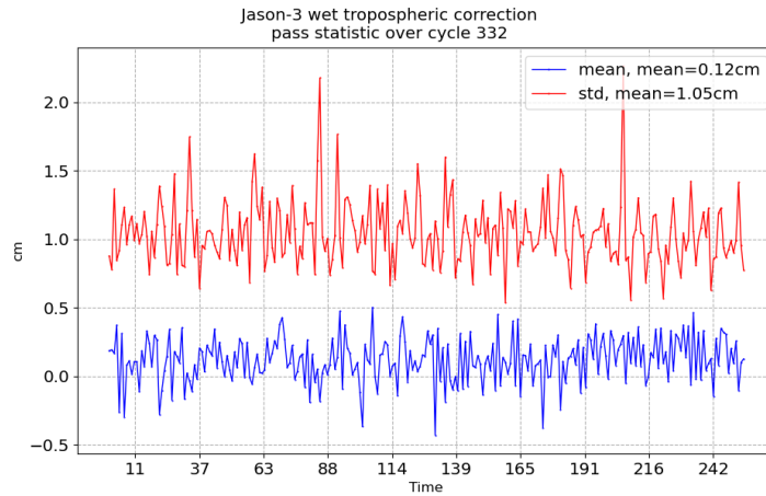
FIGURE 11 – Pass monitoring of wet troposphere differences between radiometer and ECMWF model for Jason-3 cycle 332
