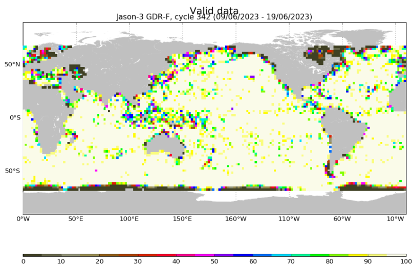
FIGURE 3 – Percentage of valid measurements for cycle 342.
