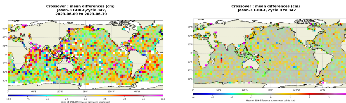
FIGURE 13 – Mean SSH at crossovers for cycle 342 (left) and over the whole Jason-3 period (right).
