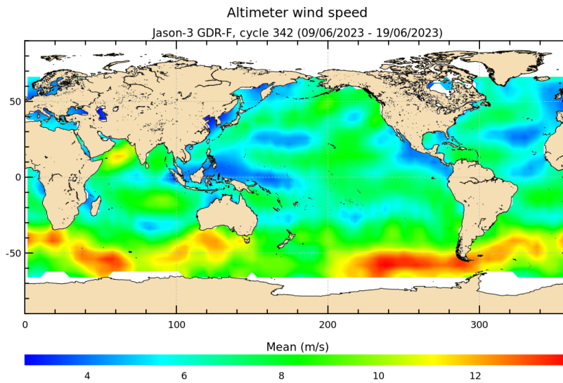
FIGURE 9 – Altimeter wind speed for cycle 342.
