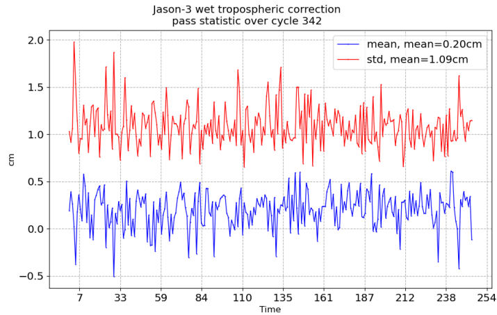
FIGURE 11 – Pass monitoring of wet troposphere differences between radiometer and ECMWF model for Jason-3 cycle 342
