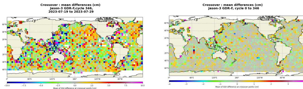
FIGURE 13 – Mean SSH at crossovers for cycle 346 (left) and over the whole Jason-3 period (right).
