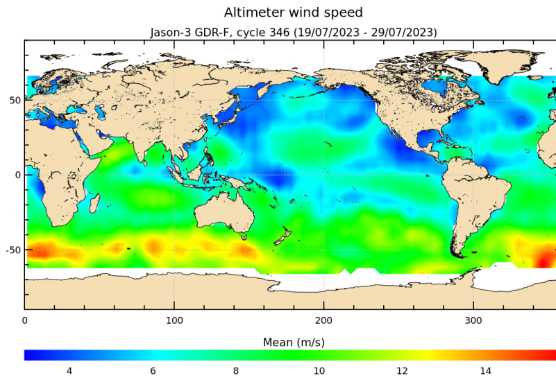
FIGURE 9 – Altimeter wind speed for cycle 346.
