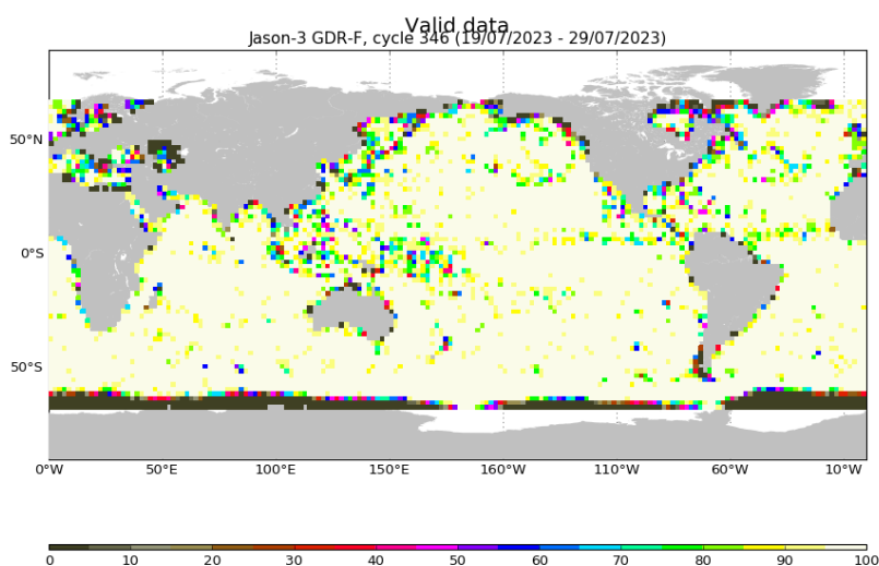
FIGURE 3 – Percentage of valid measurements for cycle 346.
