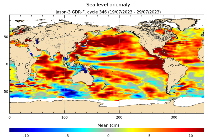
FIGURE 18 – Sea level anomaly relative to MSS for cycle 346.
