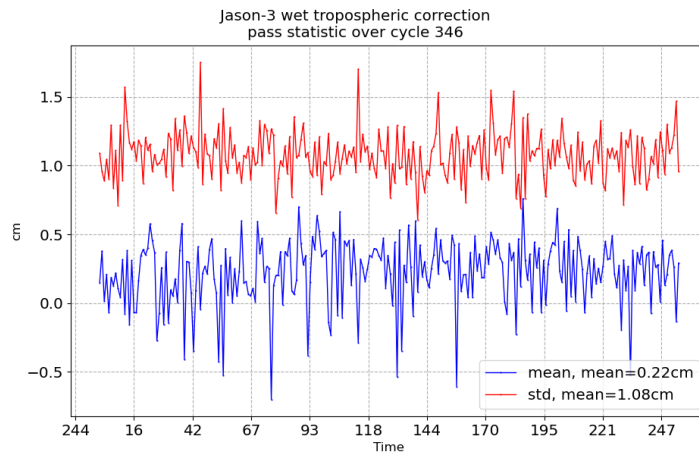
FIGURE 11 – Pass monitoring of wet troposphere differences between radiometer and ECMWF model for Jason-3 cycle 346
