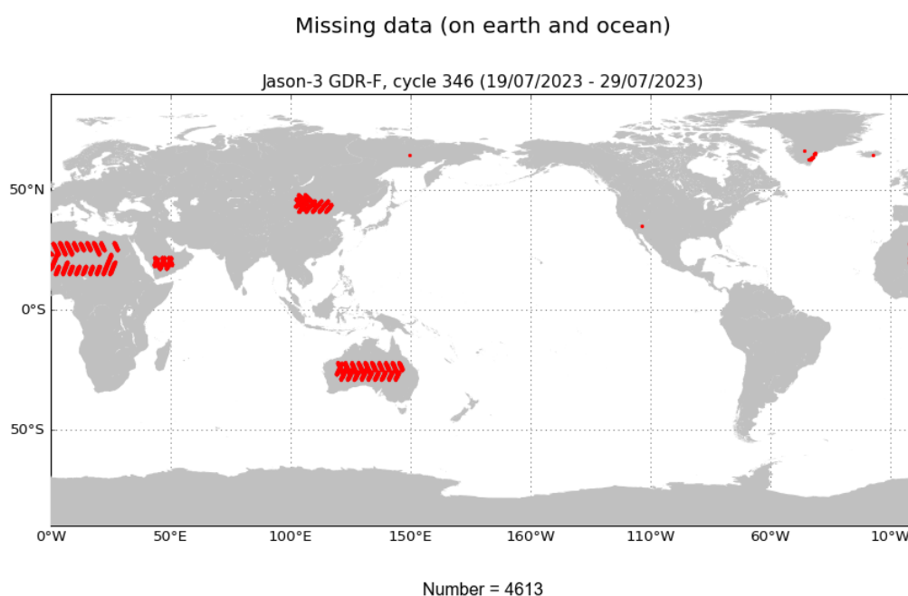
FIGURE 1 – Missing measurements for cycle 346.
