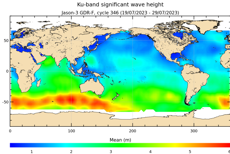
FIGURE 5 – Significant wave height for cycle 346.
