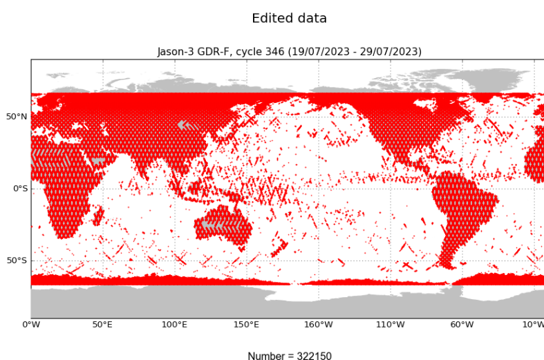
FIGURE 2 – Edited measurements for cycle 346.
