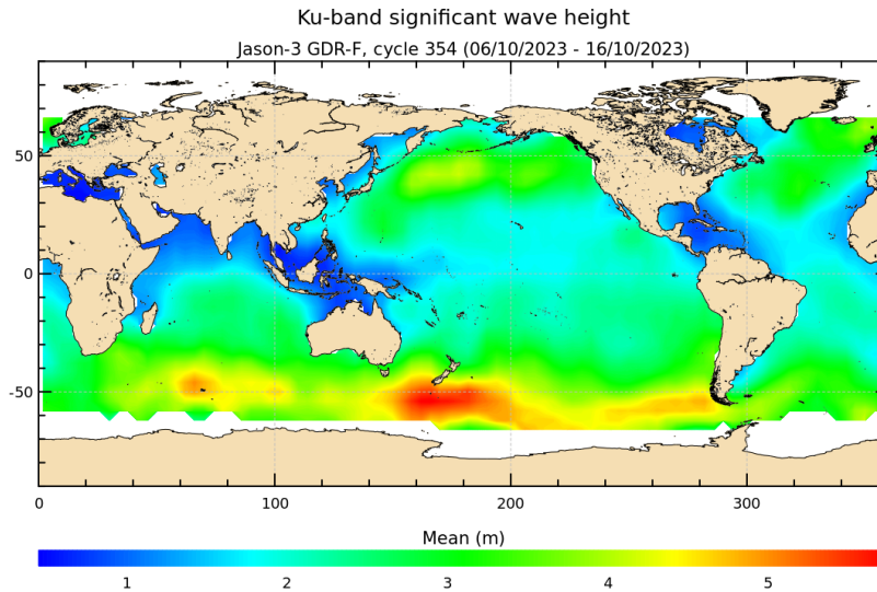
FIGURE 5 – Significant wave height for cycle 354.
