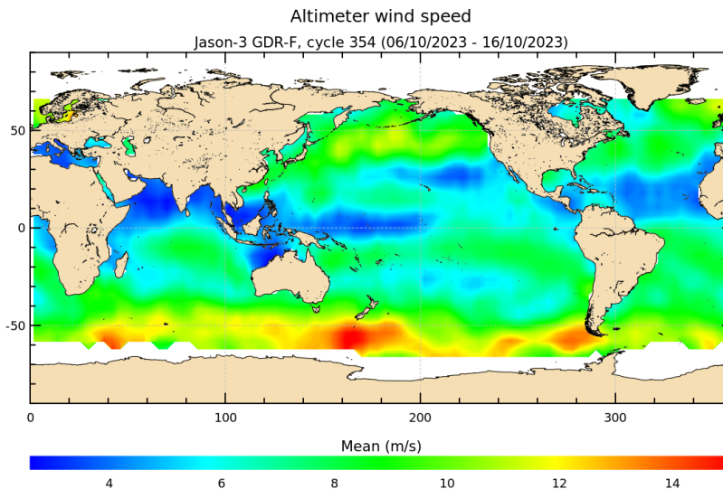
FIGURE 9 – Altimeter wind speed for cycle 354.
