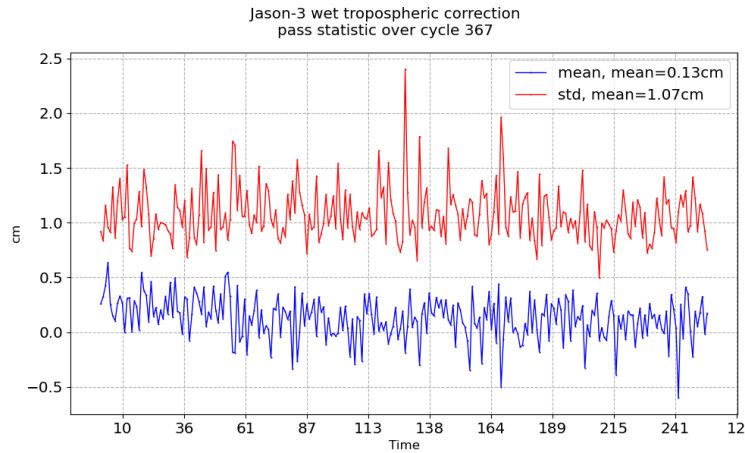
FIGURE 11 – Pass monitoring of wet troposphere differences between radiometer and ECMWF model for Jason-3 cycle 367
