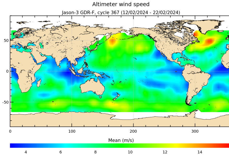
FIGURE 9 – Altimeter wind speed for cycle 367.
